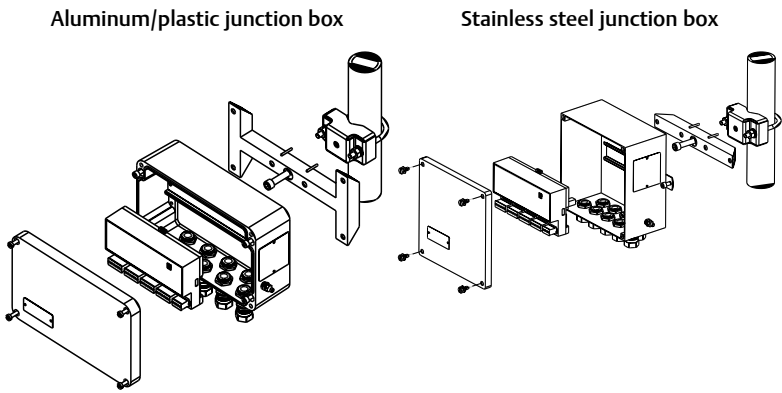
Figure 2-6: Mounted on a Vertical Pipe
