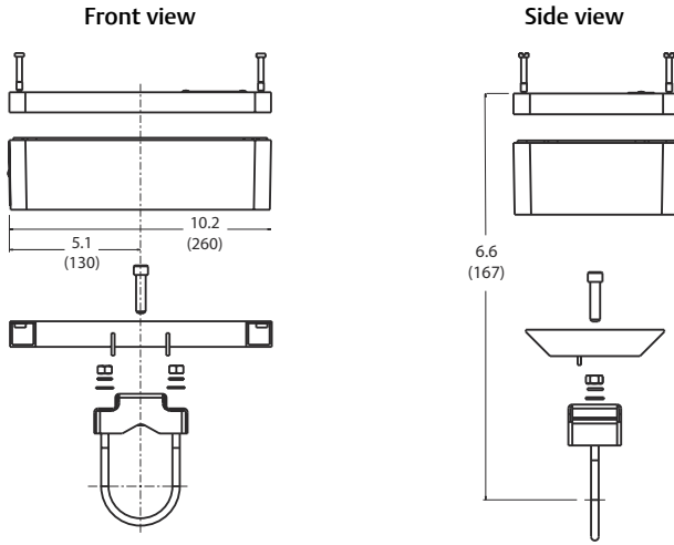
Figure 2-4: Aluminum/Plastic Junction Box
