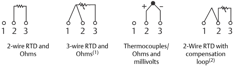
Figure 3-3: Sensor Wiring Diagrams
