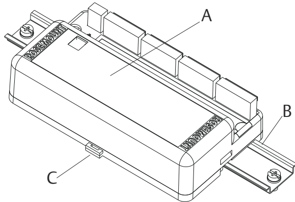
Figure 2-1: Mounting the Rosemount 848T to a DIN Rail
