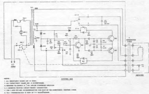
Plate 2 — SCHEMATIC
