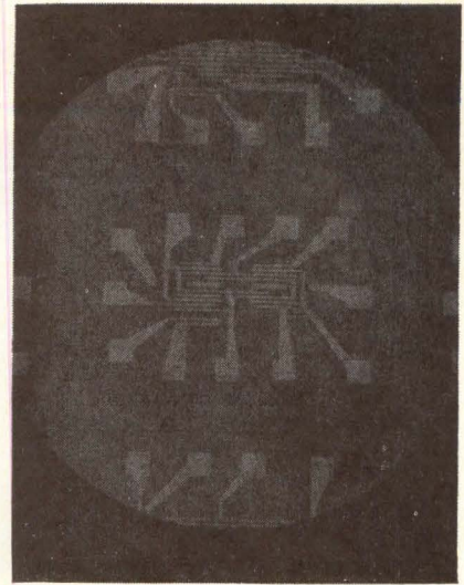
(b) Push-pull cell of Fig. 5.
