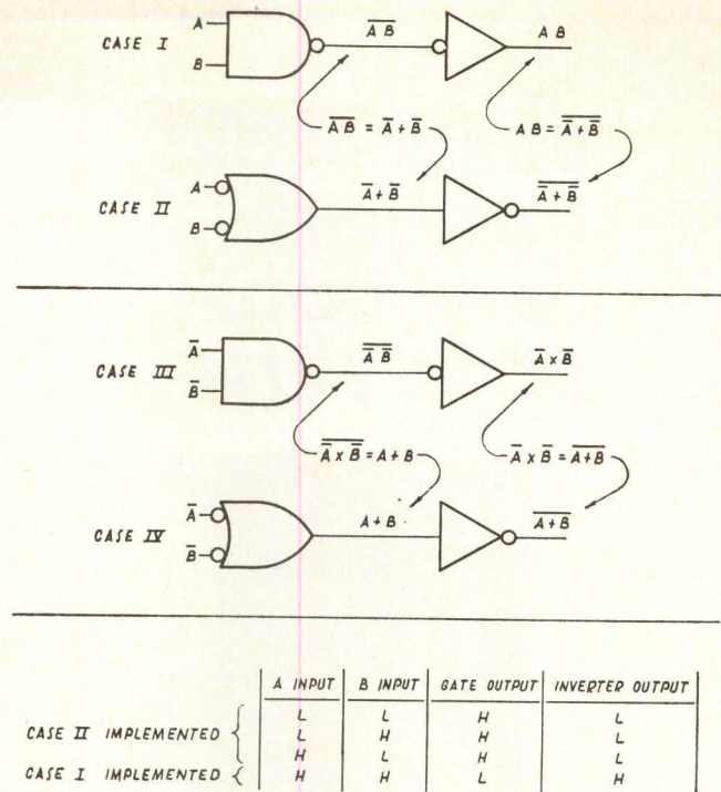
TRUTH TABLE OF A #94G LOGIC GATE, CASE I & CASE II
