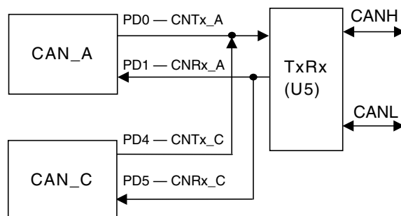
Figure 6. Sample CAN module hardware setup
