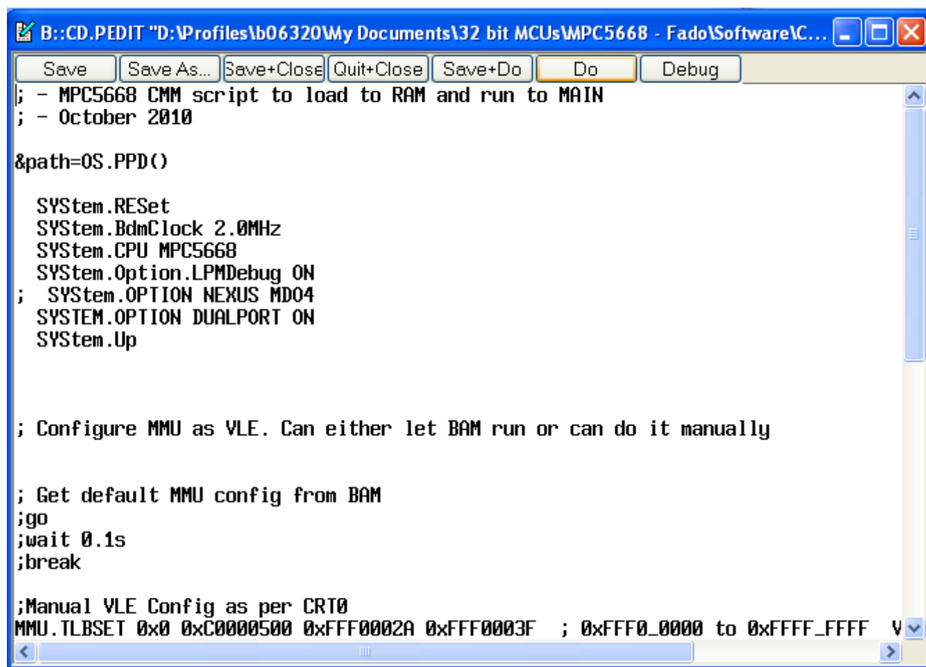
Figure 4. MPC5668 CMM script
