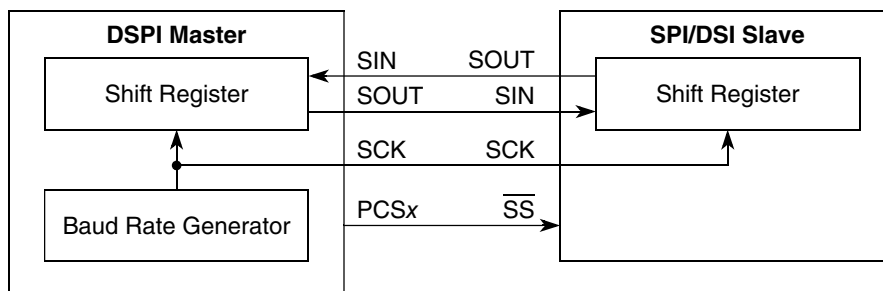
Figure 5. DSPI connections for SPI transfer
