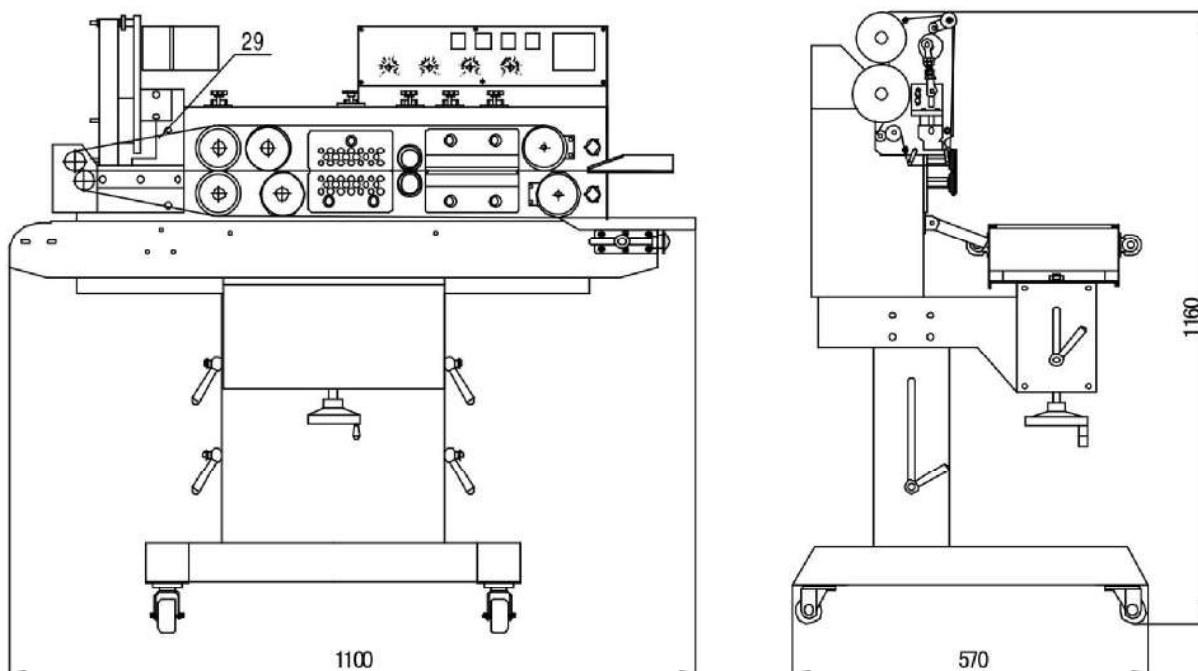
Figure 2. FRS-1120W Band Sealer (29) Hot Stamp Imprinter
