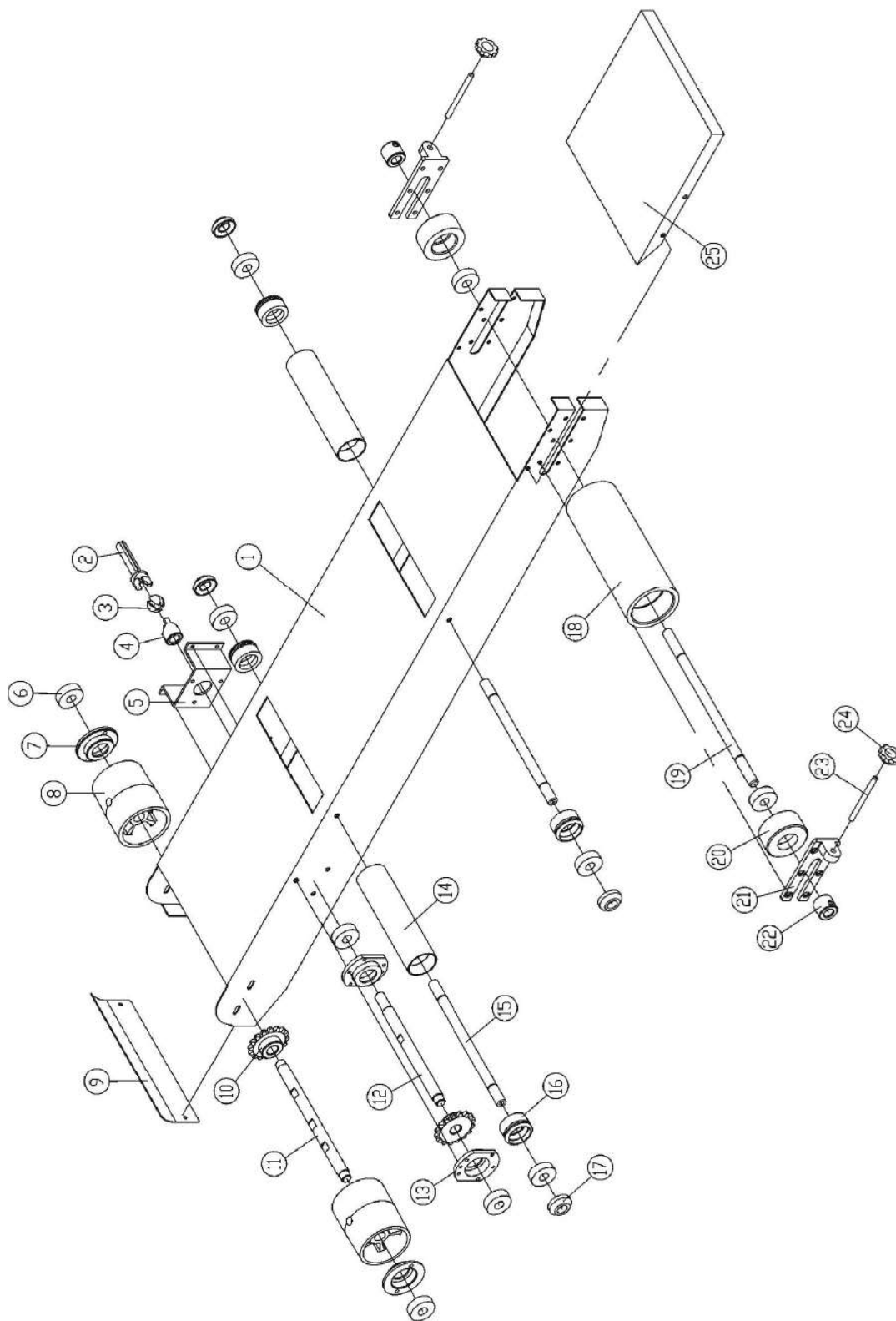
Figure 36. Conveyor Table
