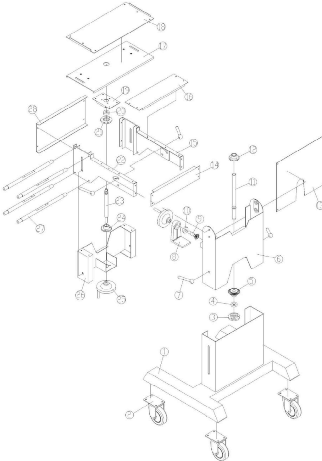
Figure 41. Sealer Rack
