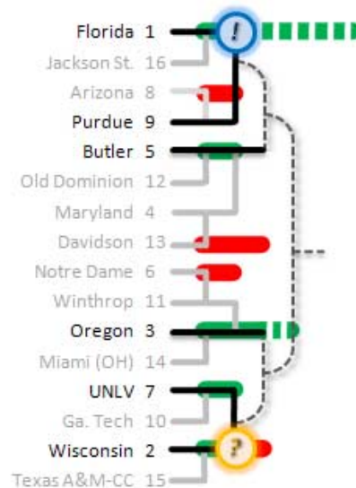
Figure 4. AdaptiviTree layout of a bracket. A player’s picks are superimposed on the results with a colored overlay. Icons are overlaid to indicate two possible scenarios of interest.
