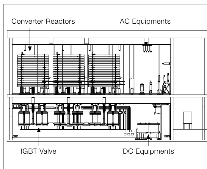
Troll A 3 & 4.
