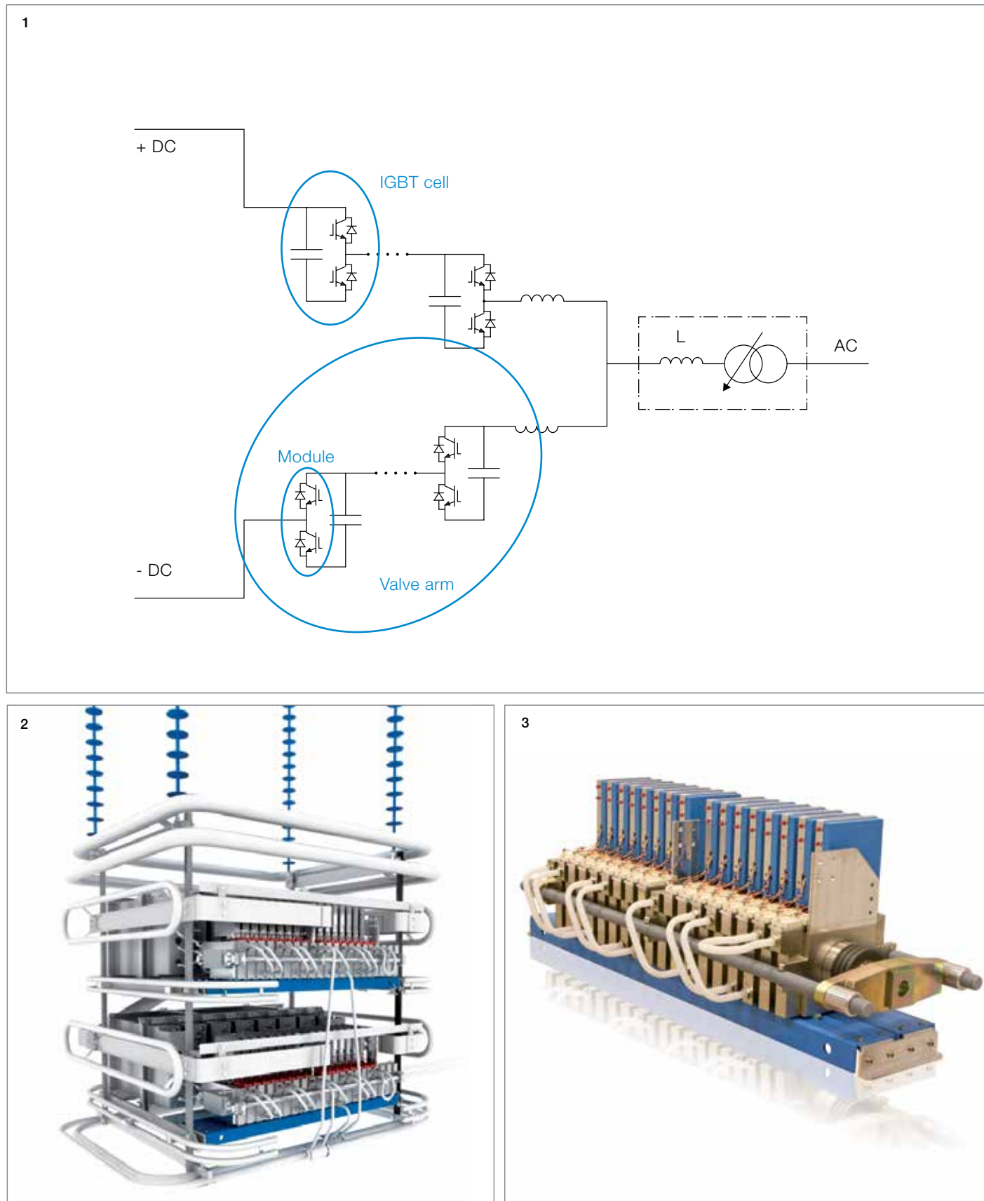
1 Principle schematic of an HVDC Light® converter (one phase) | 2 One double cell | 3 One IGBT module.
