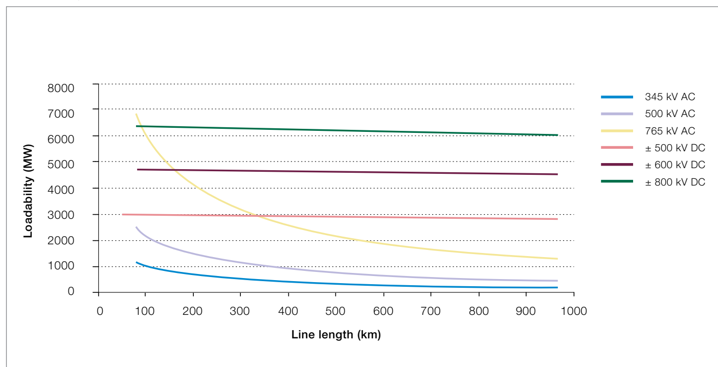
Line loadability vs. distance for AC and DC lines.
