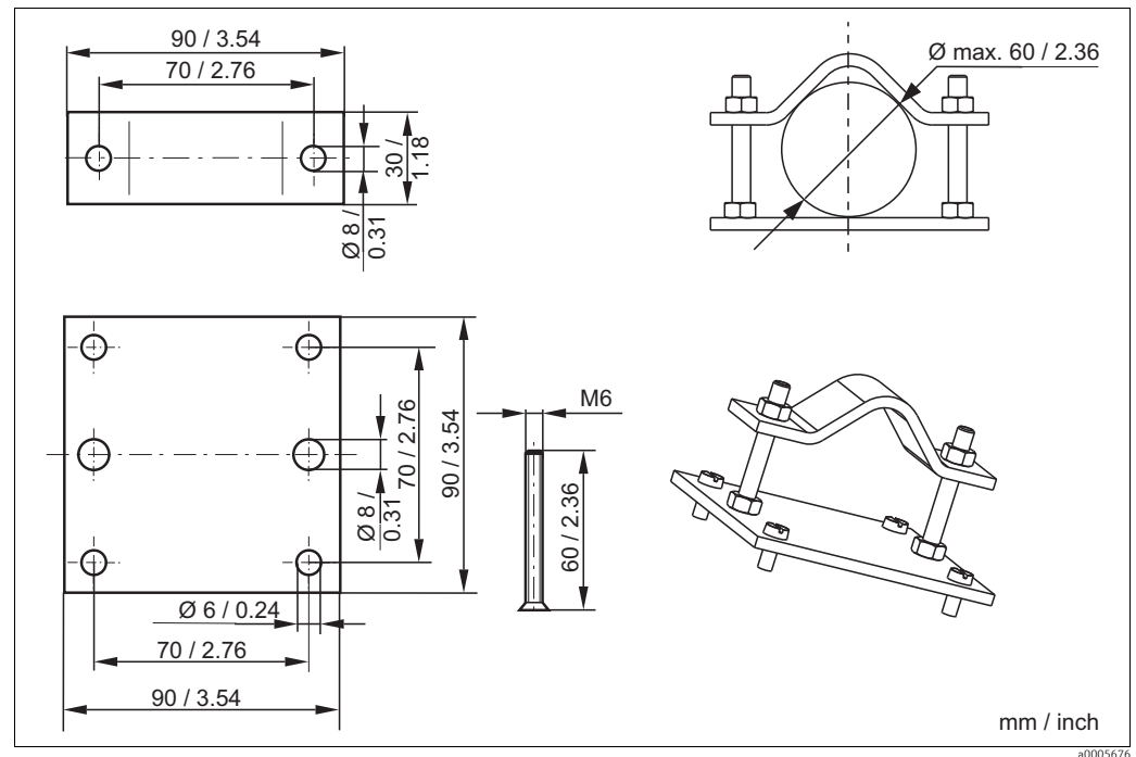
Fig. 35: Post mounting kit
