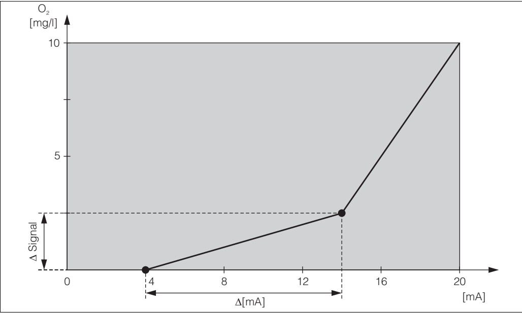
Fig. 24: User-defined current output characteristic (example)
