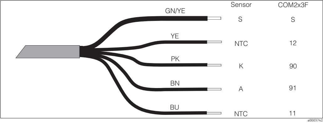
Fig. 12: Measuring cable COK21
