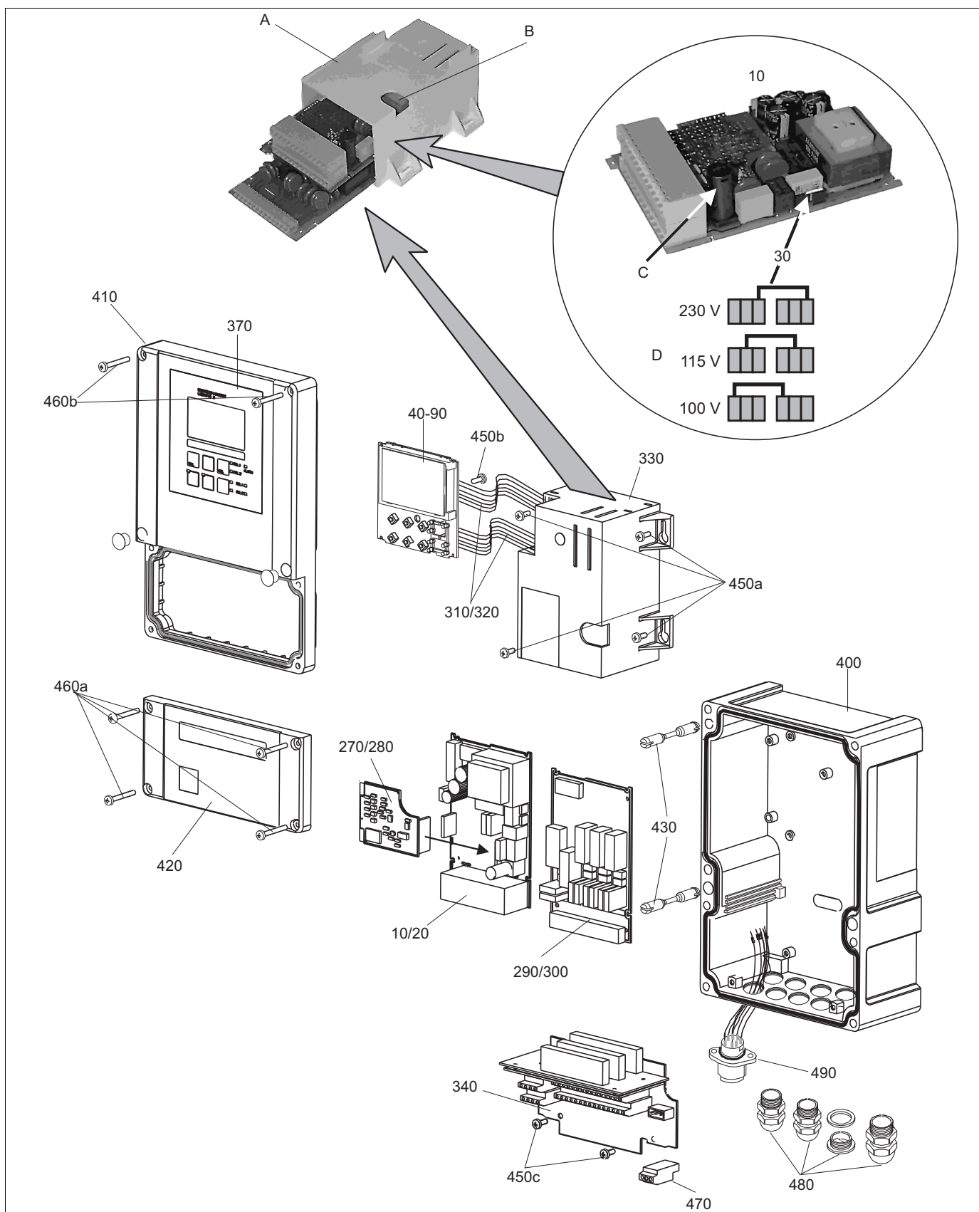
Fig. 32: Exploded view drawing of field instrument
