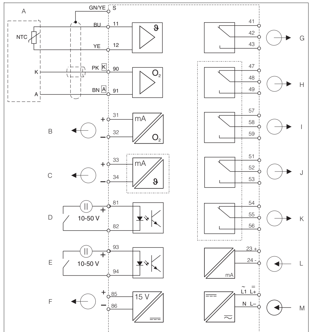
Fig. 9: Electrical connection of the transmitter
