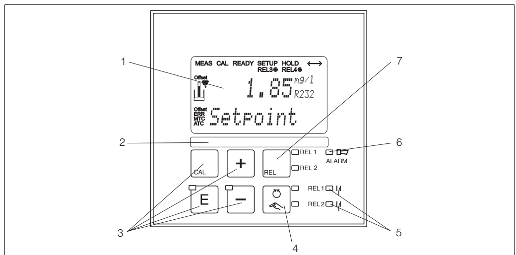
Fig. 16: Operating elements
