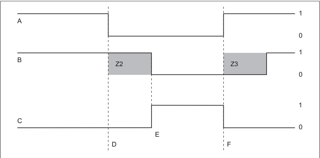
Fig. 21: Alarm signalling and dosing switch-off by the main stream A Flow in main stream F Flow restoration B Relay contacts of PID controller Z2 Delay for controller switch-off, see field Z2 C Alarm relay Z3 Delay for controller switch-on, see field Z3 D Flow below switch-off limit Z4 or flow failure 0 Off E Flow alarm 1 On
