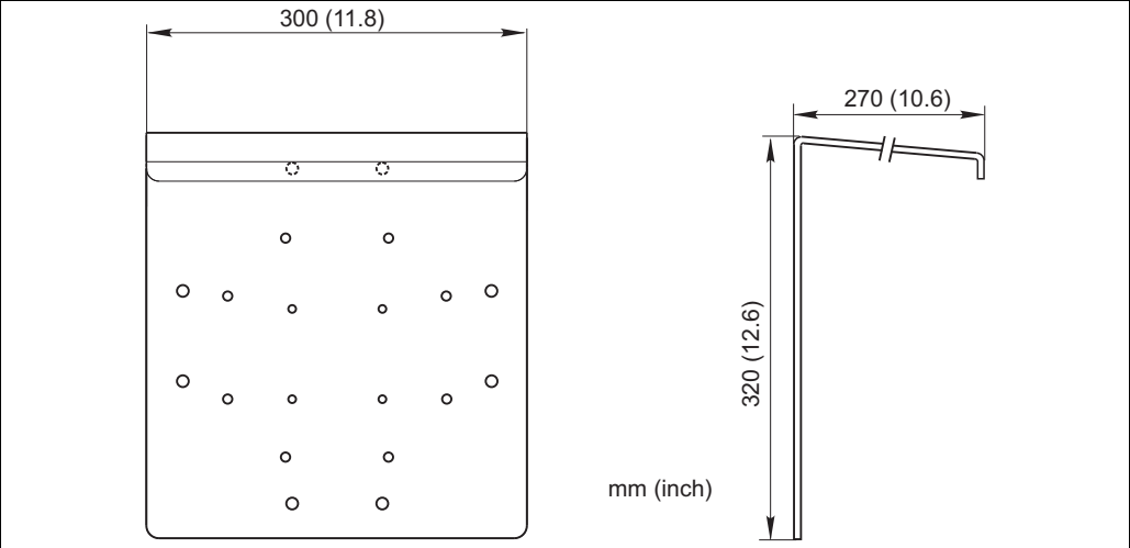
Fig. 33: Weather protection cover for field devices
