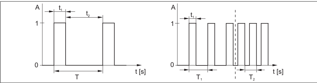
Fig. 27: Signal of a pulse-length modulated controller contact (left) and of a pulse-frequency modulated controller contact (right) A Contact 1 = on, 0 = off T Period length B Time [s] t_1 = t_{\text{on}} t_2 = t_{\text{off}} T_1 T_2 Impulse period length (impulse freq. 1/T_1 and 1/T_2 )
