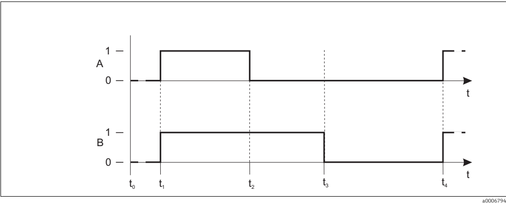
Fig. 29: Correlation of cleaning time, pause time and hold dwell period A Wiper and/or spray cleaning system t_0 Normal mode B Hold function t_1 Cleaning start 0 Inactive t_2-t_1 Cleaning time 1 Active t_3-t_2 Clean hold dwell period (0 to 999 s) t_4-t_3 Pause time between two cleaning intervals (1 to 7200 min)
