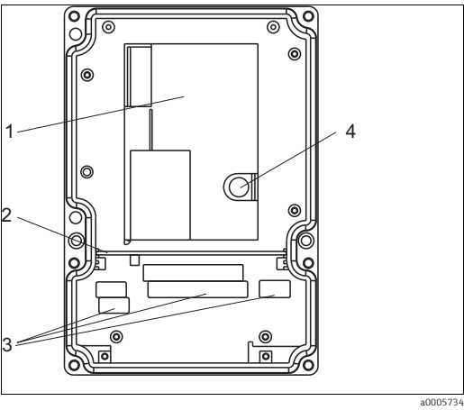
Fig. 3: View into the field housing
