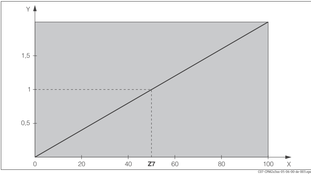
Fig. 23: Multiplying feedforward control Y Gain K_{inff} X Current input signal [%] Z7 Input value, when gain K_{inff} = 1
