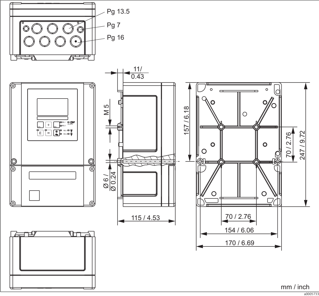
Fig. 2: Field instrument
