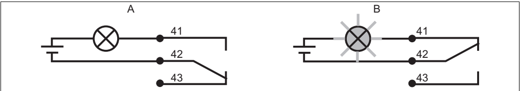
Fig. 14: Recommended fail-safe switching for the alarm contact A Normal operating status B Alarm condition
