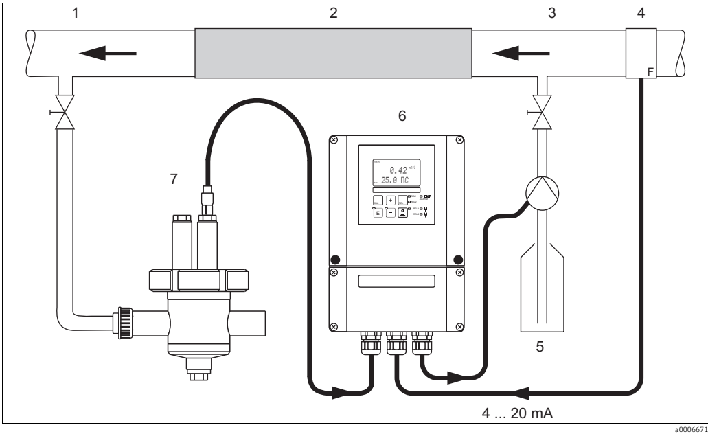
Fig. 22: Arrangement example for feed forward control of the flow rate in the main stream to the PID controller 1 Measuring water extraction point 5 Injection medium 2 Static mixer 6 Liquisys M COM253F 3 Injection points 7 CPA240 with COS21 4 Flowmeter
