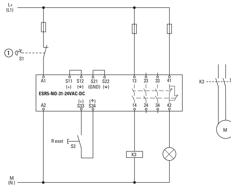
Figure 4: Single-channel emergency stop monitoring
