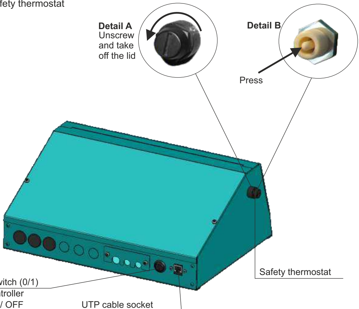
Picture – Safety thermostat
