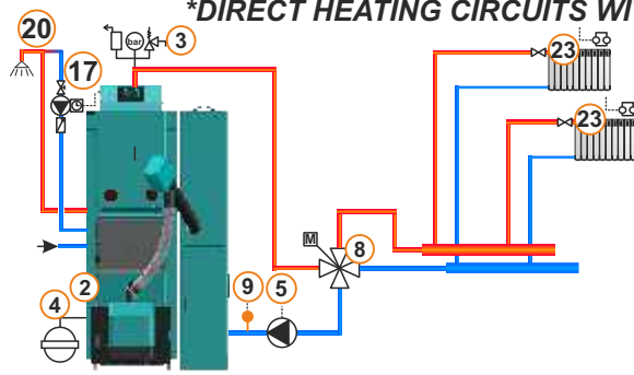
*DIRECT HEATING CIRCUITS WITHOUT PUMPS
