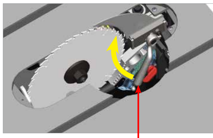
pull handle upward to release clamp
