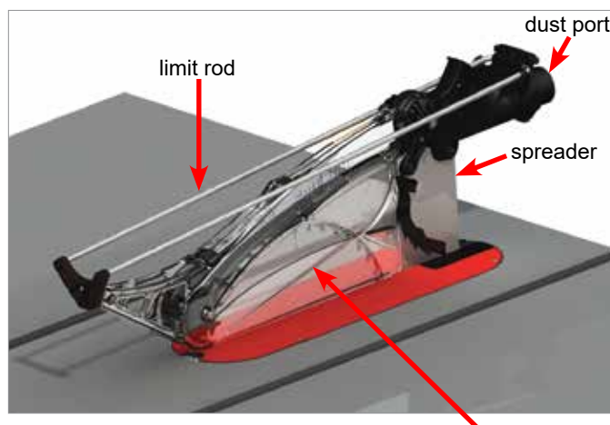
Fig. 33 blade guard shell
