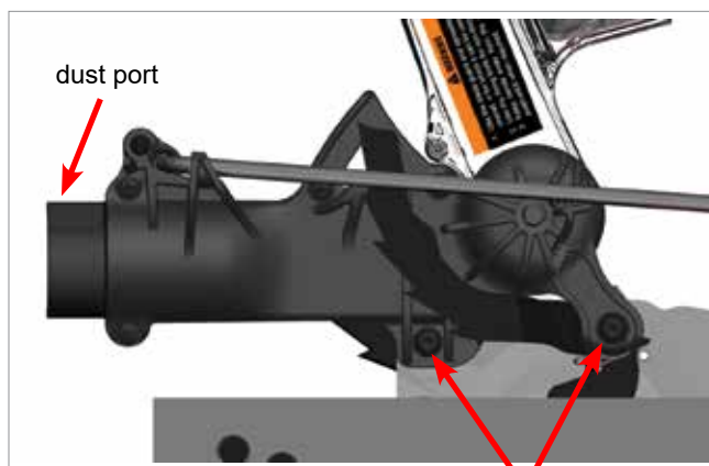
Fig. 83 loosen these two bolts
