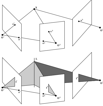
Figure 5: Trifocal geometry . Rays backprojected from corresponding image points in the first and second view intersect, and thus determine, the 3D point. The position of the corresponding point in the third view is computed by projecting this 3D point onto the image. Similarly lines backprojected from the first and second image intersect in the 3D line, the projection of this line in 3-space to the third image determines its image position.
