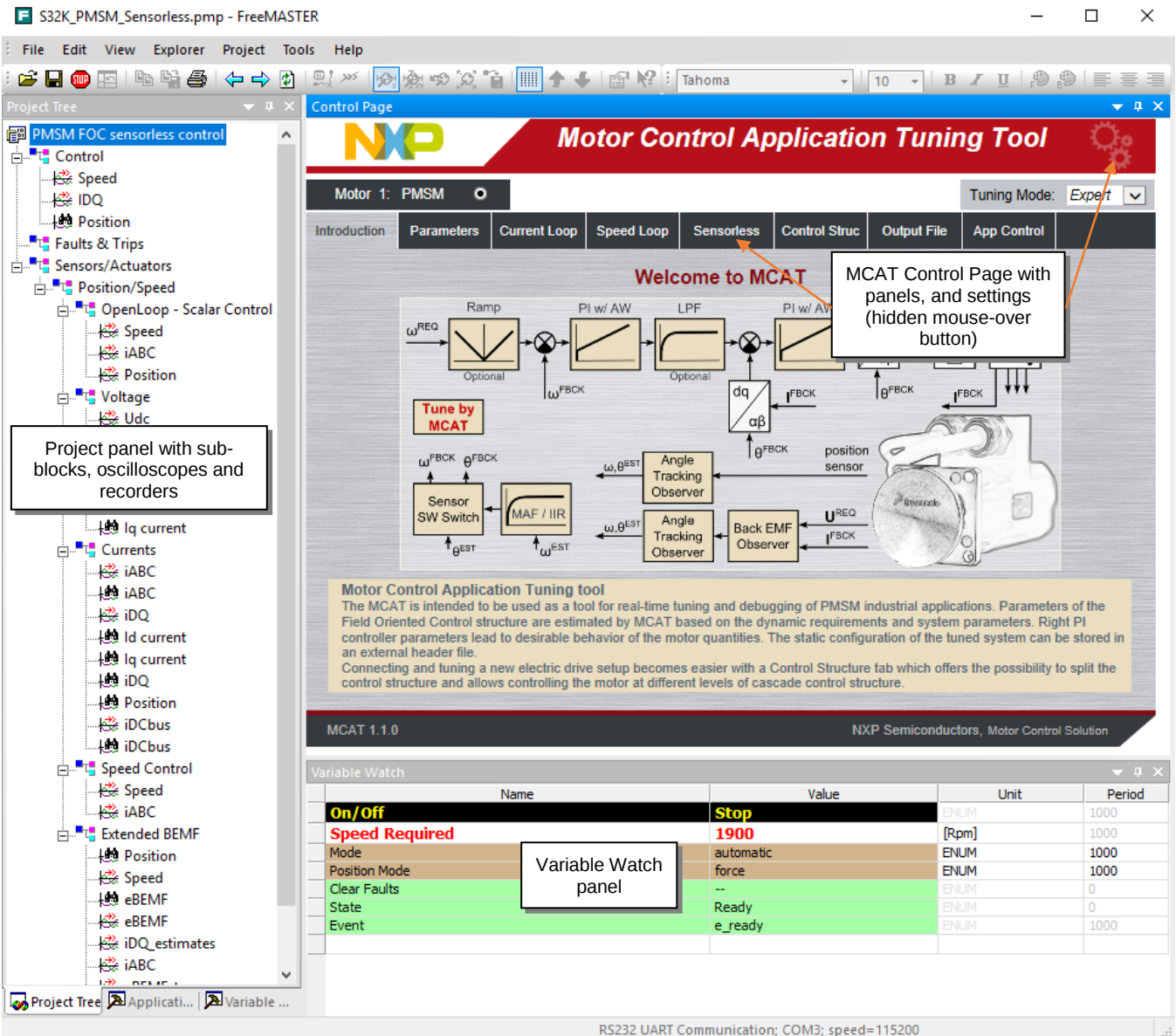
Figure 42. FreeMASTER and Motor Control Application Tunning Tool
