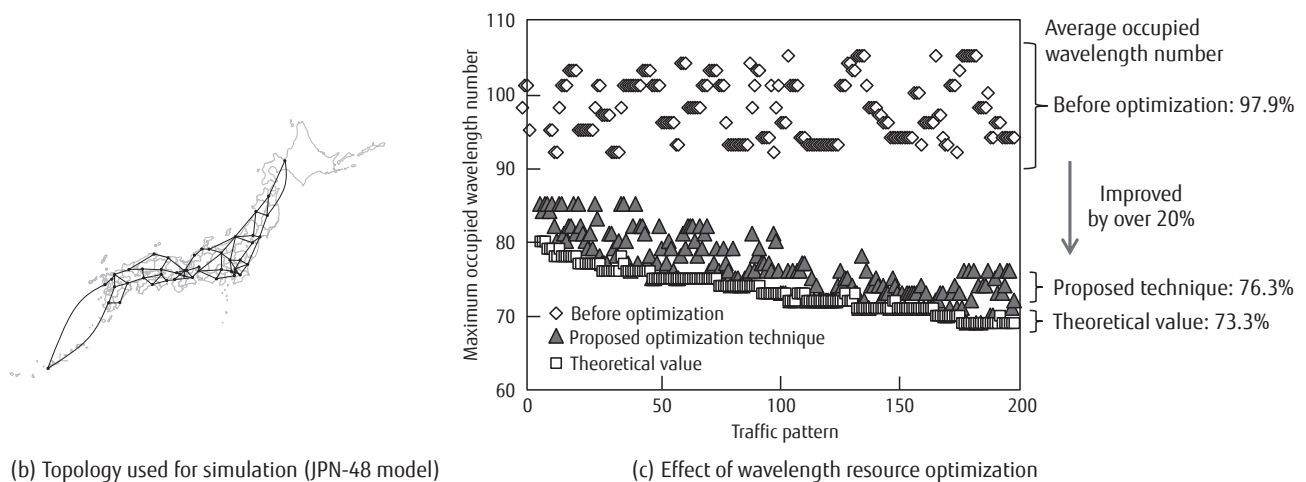
Figure 3 Optimization of optical wavelength resources in optical network.
