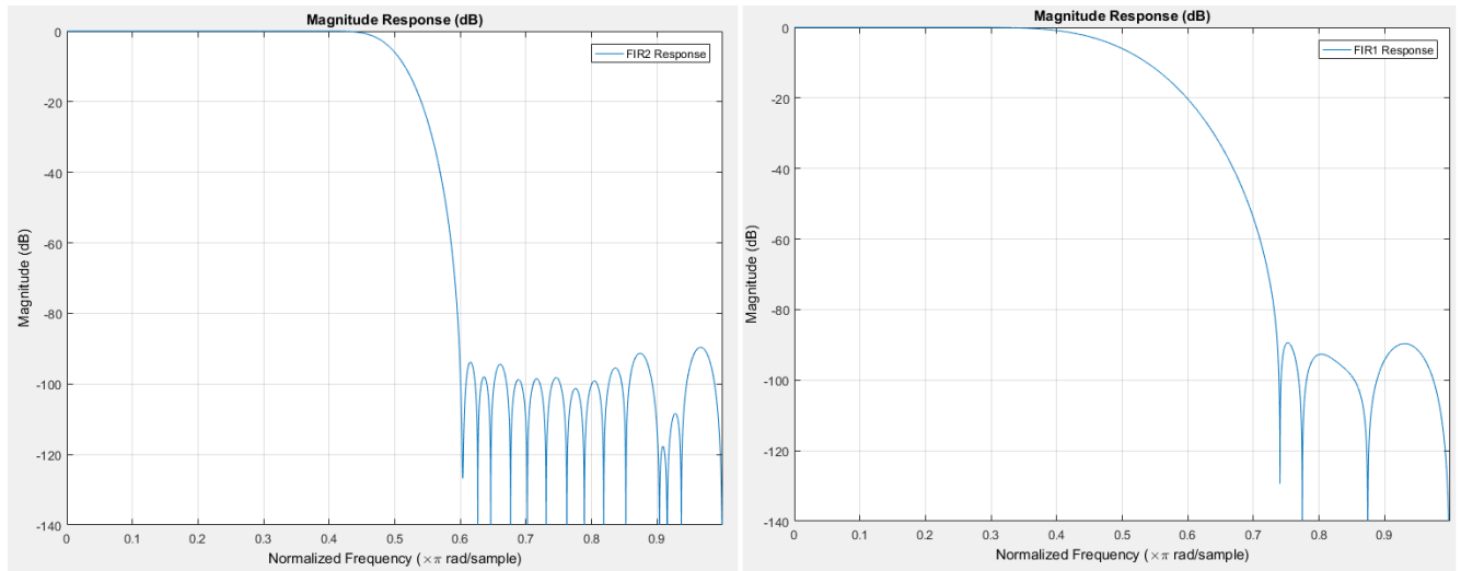
Figure 18: FIR2 and FIR1 Frequency Response
