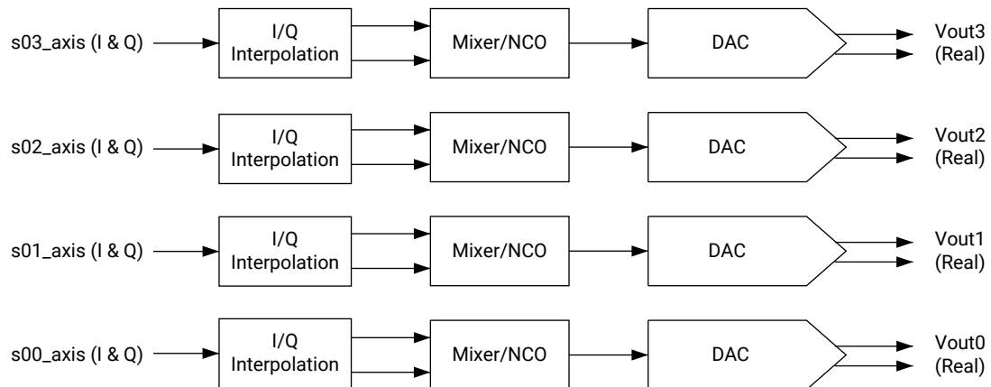
Figure 64: RF-DAC I/Q Input to Real Output
