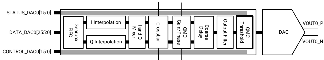
Figure 44: Simplified RF-DAC Functionality Block Diagram
