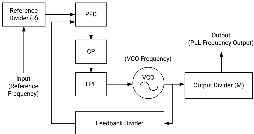
Figure 72: PLL System
