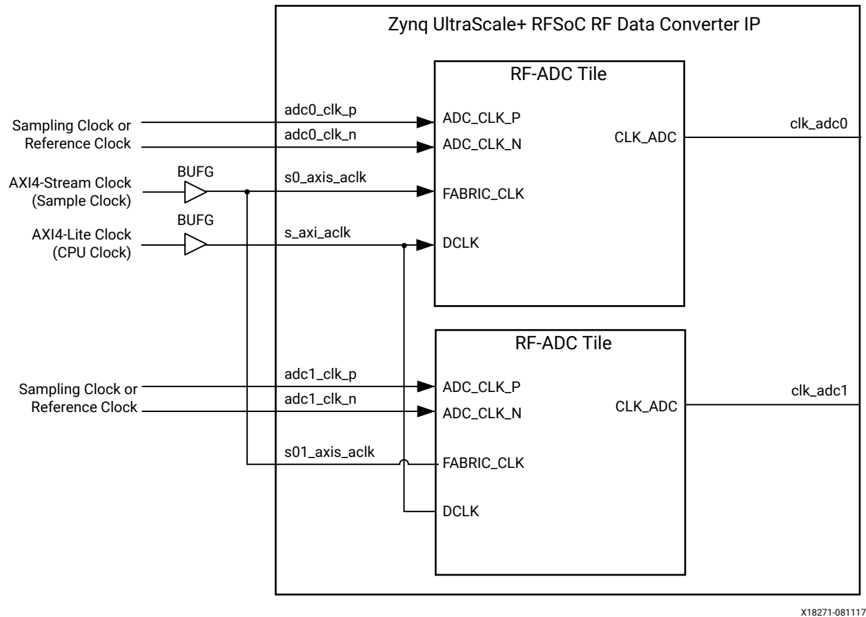
Figure 76: IP Core Clocking
