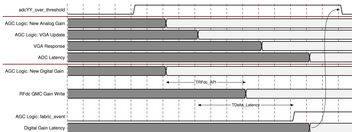
Figure 90: Example AGC Threshold Event Response
