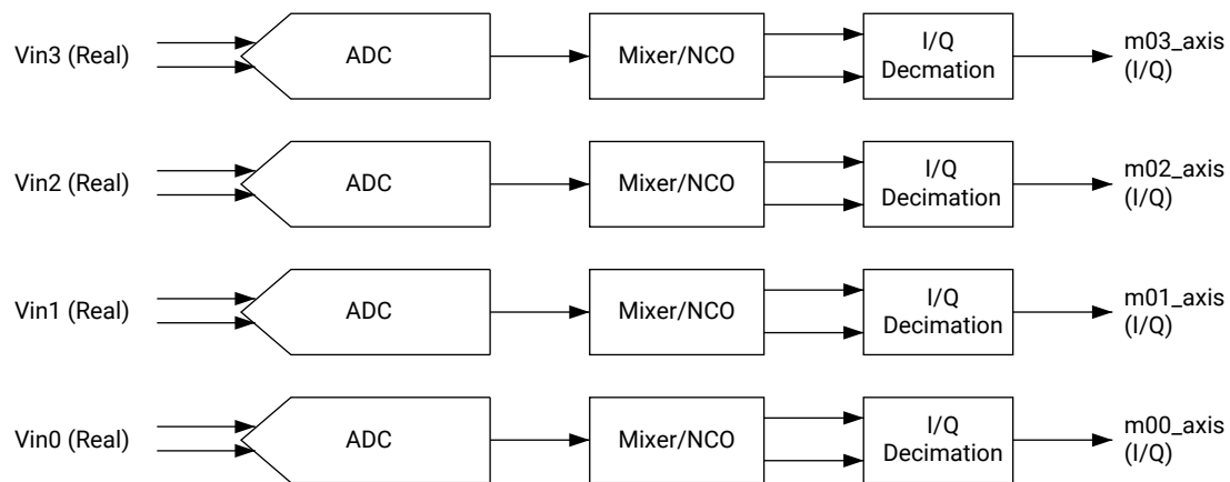
Figure 38: Quad RF-ADC Real Input to I/Q Output
