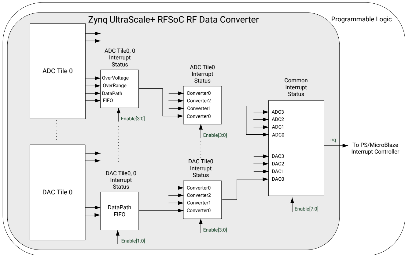
Figure 73: Interrupt Hierarchy
