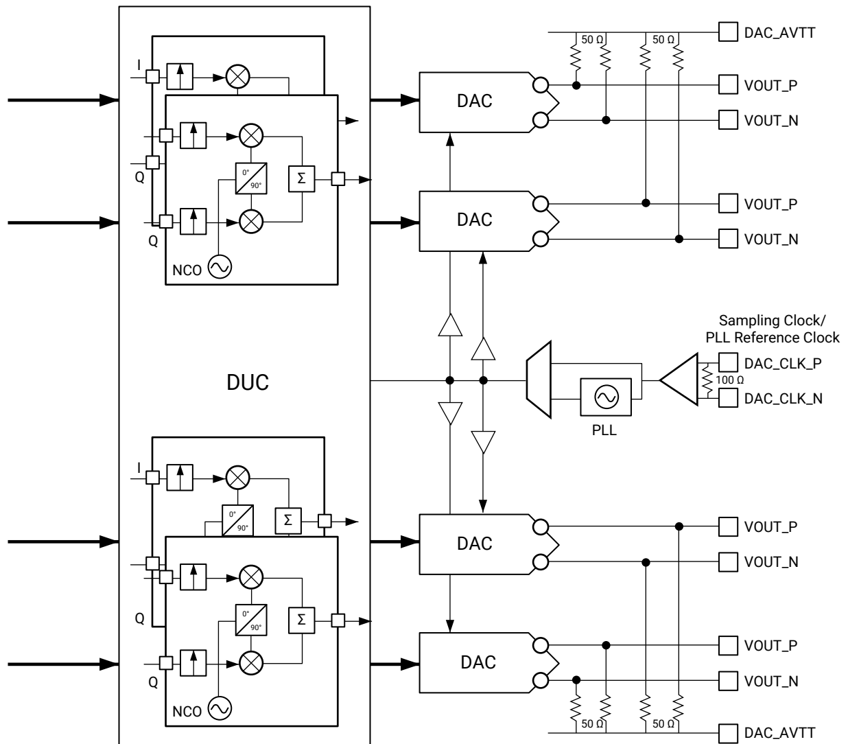
Figure 6: RF-DAC Overview
