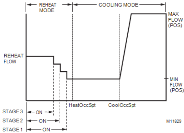
Figure 21: VAV box modes for Reheat Type Elec_ThreeStage - Proportional
