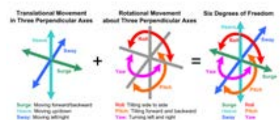
Figure 2. TARS Six Degrees of Freedom
