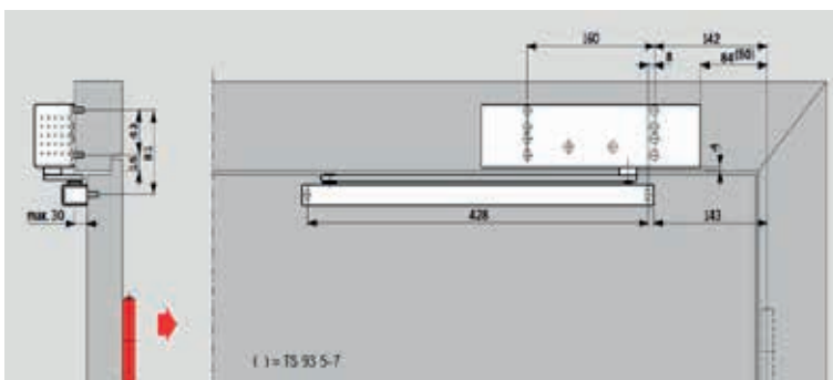
Transom fixing (overhead frame fixing) of the TS 93 B on the push side.
