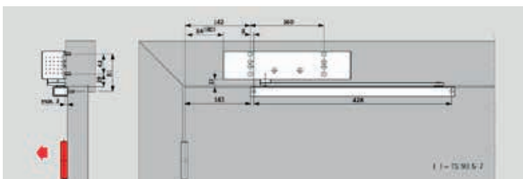
Transom fixing (overhead frame fixing) of the TS 93 G on the pull side.
