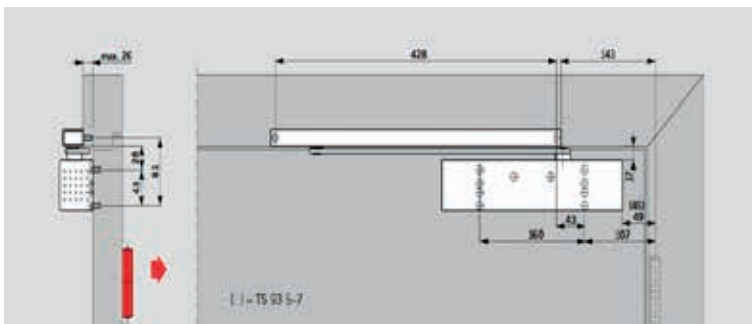
Door leaf fixing (standard installation) of the TS 93 G on the push side.
