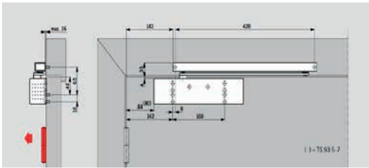
Door leaf fixing (standard arrangement) of the TS 93 B on the pull side.
