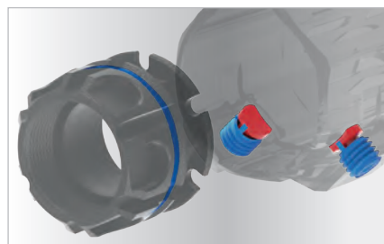
Barrel Nut Features a Precisely Machined Indexing Channel around its Circumference
