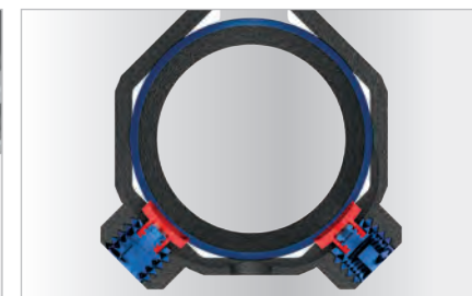
Locking Tabs, Integrated within the Locking Screws, Index Against the Barrel Nut's Channel After Being Tightened, Creating a Rigid 4-Point Steel-on-Steel Lockup
