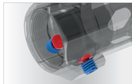
Handguard Secures to Barrel Nut Simply by Tightening the Locking Screws to their Proper Torque Value
