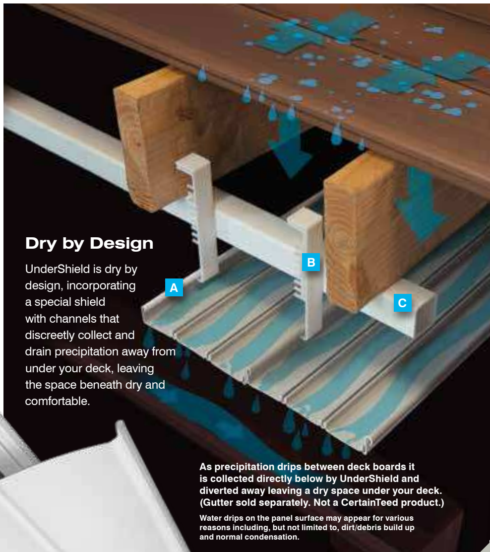
C Vinyl Grid System
