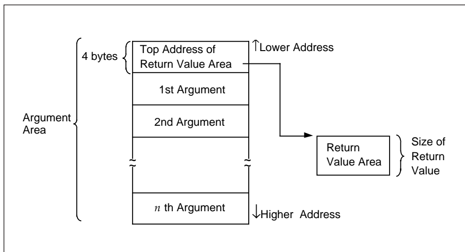
Figure 6.5 Argument Area for the Function which Returns Structure or Union
