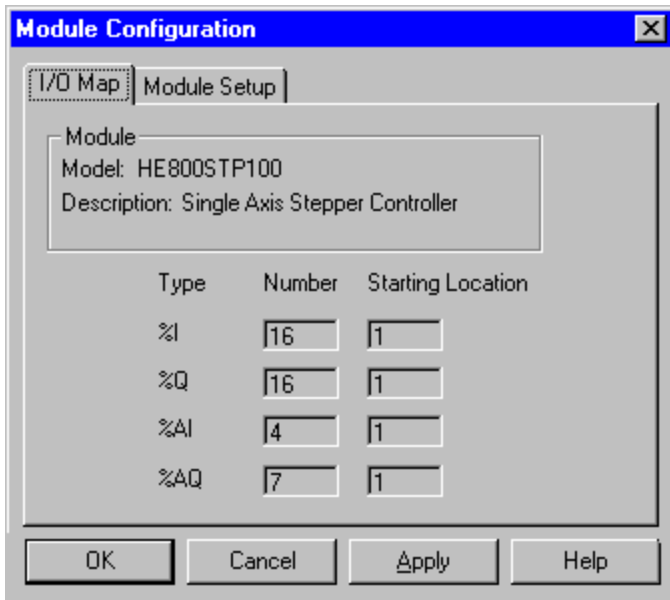
Stepper Config
