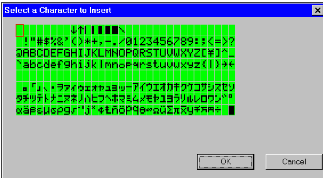
Figure 15.1 – ASCII Chart
