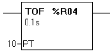
Timer OFF Delay
