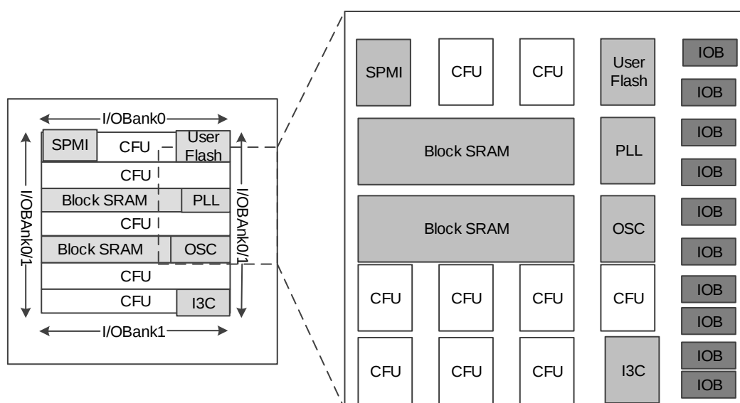
Figure 3-1 GW1NZ Architecture Overview
