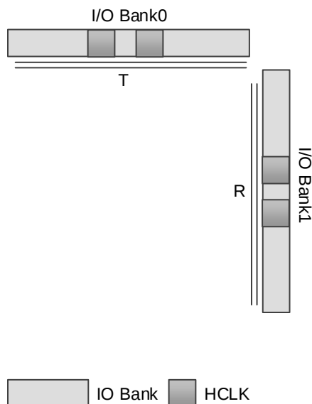
Figure 3-28 GW1NZ-1 Clock Resources
