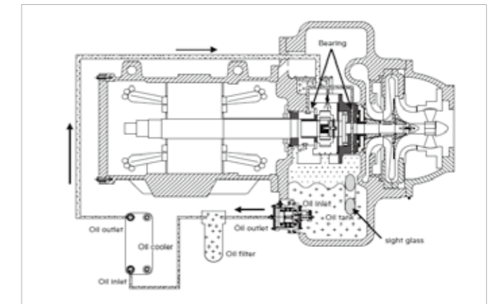
Lubrication cycle
