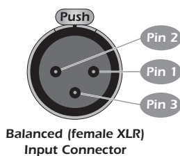
Figure 2-3: N°32 Balanced Connector Pin Assignments.
