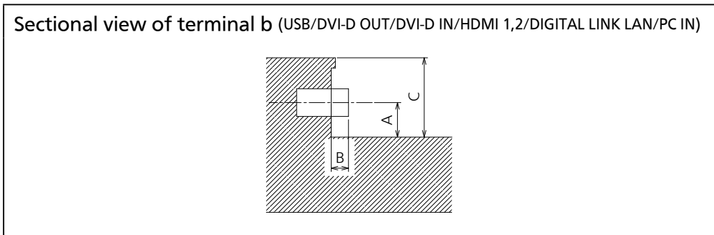
Terminal b 70SF2HU Terminal (Bottom)
