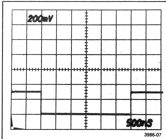
Fig. 4-5 Horizontal Sync Width
