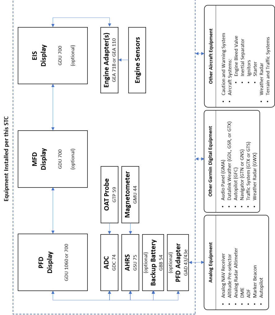
Figure 1 TXi System Overview
