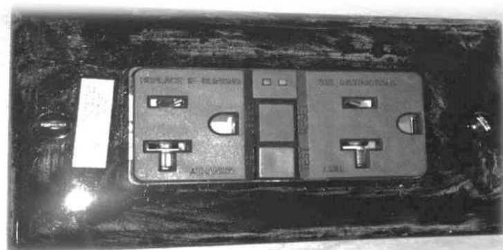
Figure 9-5: GFCI Receptacle
