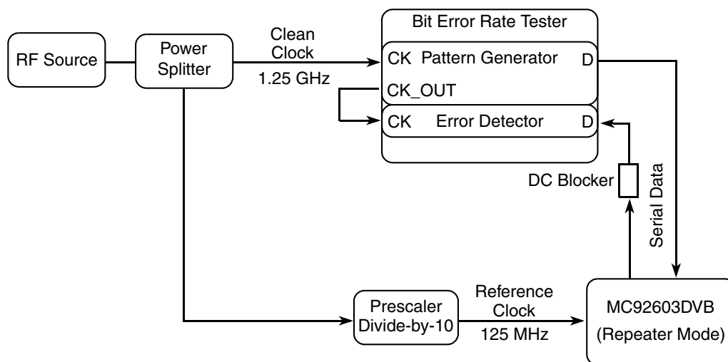
Figure 4-1. Full-Speed Serial Link Test Setup
