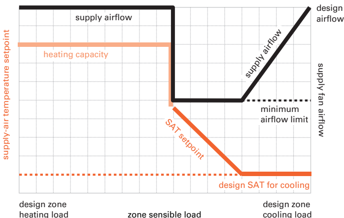
Figure 3. Example SZVAV control with variable-speed fan and constant airflow when heating
