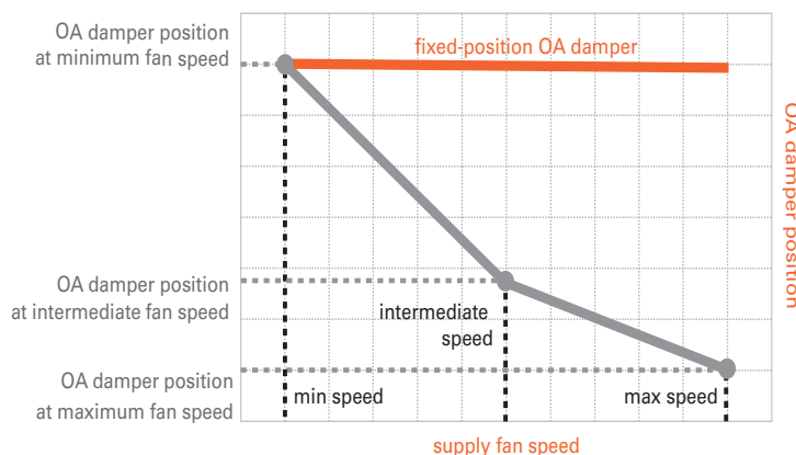
Figure 6. Proportional control of OA damper
