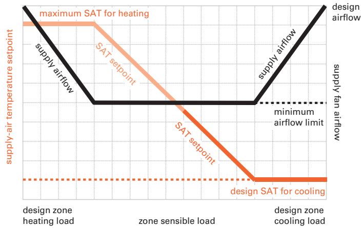
Figure 2. Example SZVAV control with variable-speed fan
