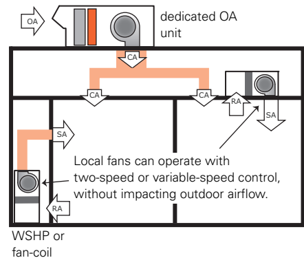
Figure 9. Conditioned OA delivered directly to each zone
