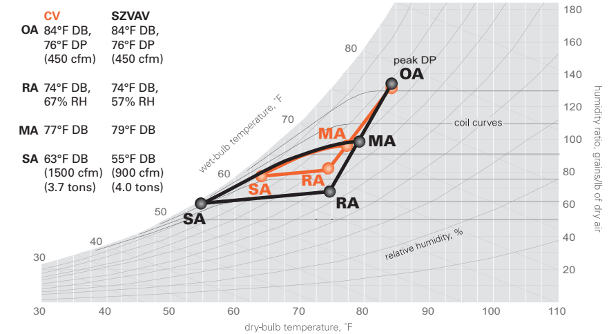
Figure 11. Improved dehumidification at part load for an example classroom in Jacksonville, FL
