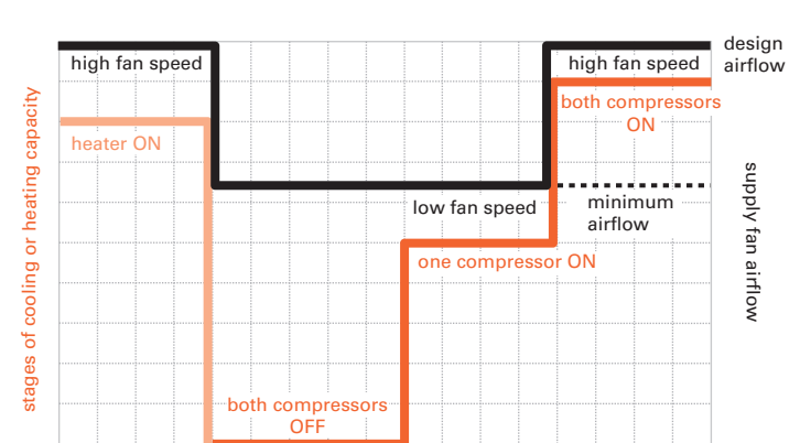
Figure 4. Example SZVAV control with two-speed fan
