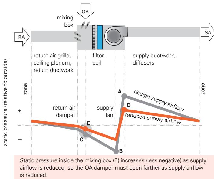
Figure 5. Need for ventilation control in SZVAV system
