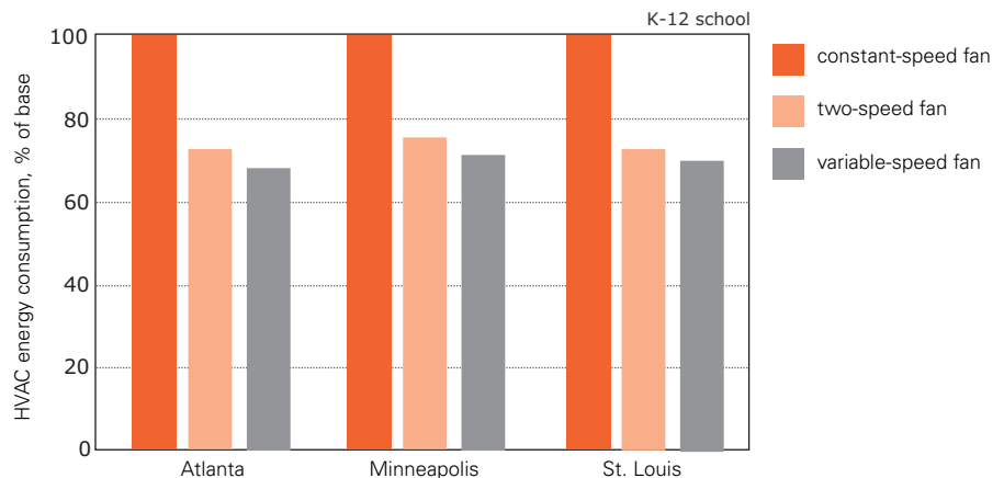
Figure 10. Example energy savings from two-speed or variable-speed fan control
