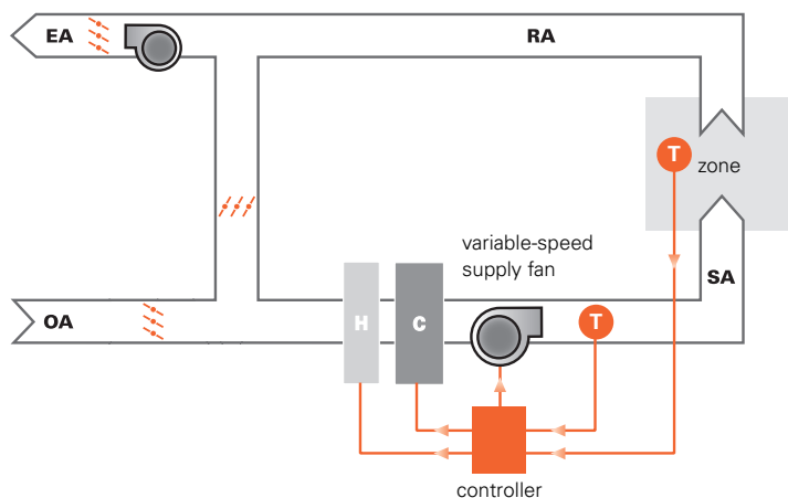
Figure 1. Single-zone VAV system
