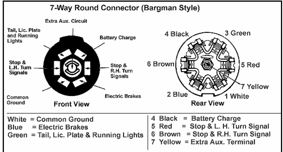
Figure 7-18. Seven-Pin Towing Connector
