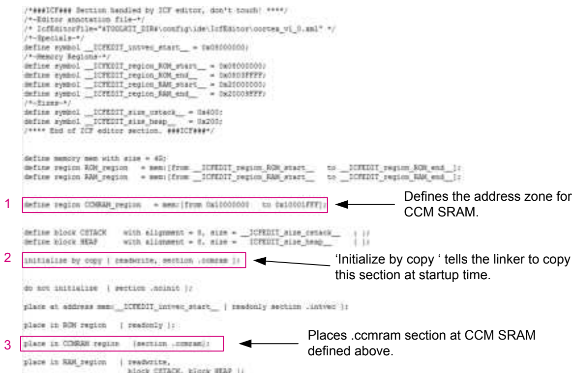
Figure 3. IAR Embedded Workbench® linker update
