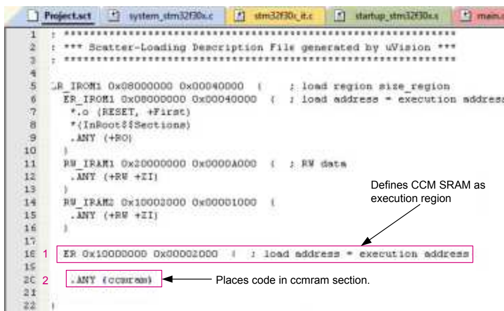
Figure 12. MDK-ARM scatter file
