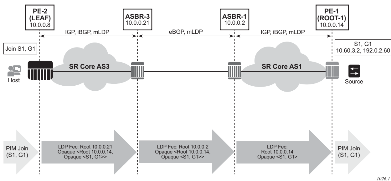
Figure 84 mLDP FEC for Inter-AS with Recursive Opaque Value
