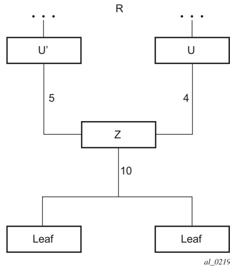
Figure 109 mLDP LSP with Backup Upstream LSR Nodes
