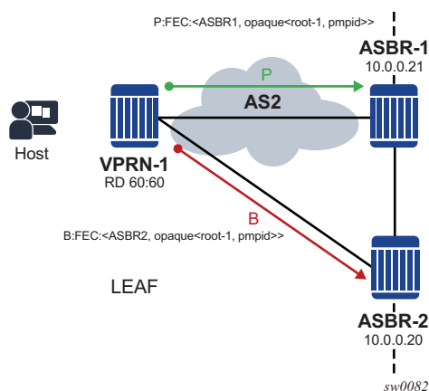
Figure 101 ASBR MoFRR Leaf Behavior
