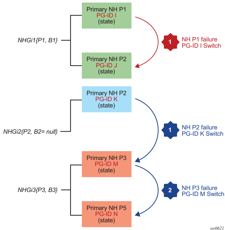
Figure 56 NHG Failover Based on PG-ID Switch
