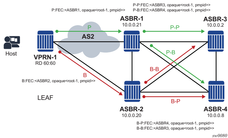
Figure 102 ASBR MoFRR ASBR Behavior
