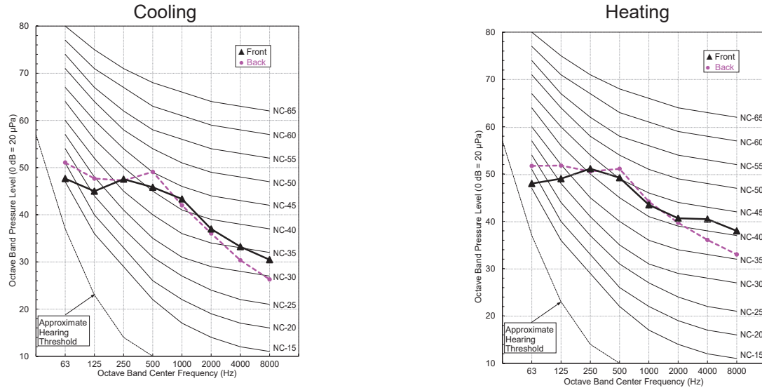
Figure 13: Sound Pressure Levels for Mega LSU180HEV2 Outdoor Units.
