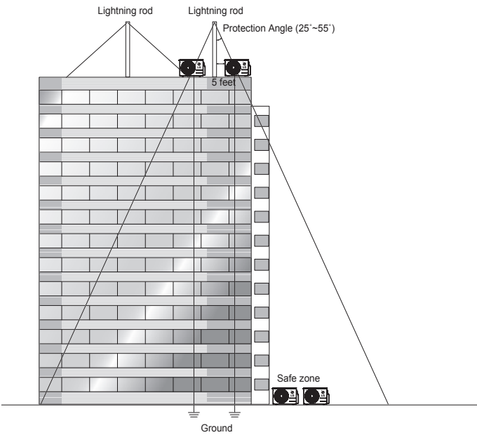
Figure 31: Lightning Protection Diagram.
