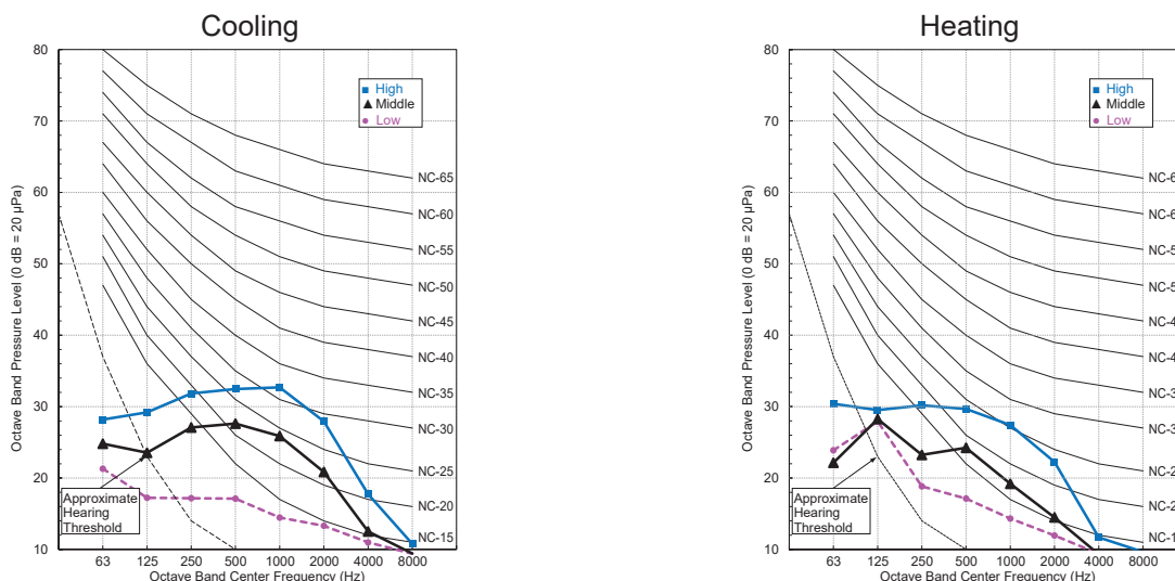
Figure 5: Sound Pressure Levels for Mega LSN090HEV2 Indoor Units.
