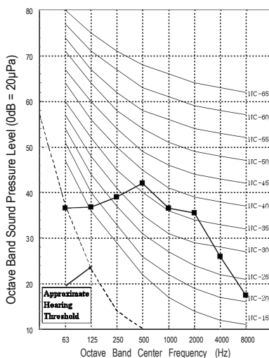
Figure 9: Sound Pressure Levels for Mega 115V Indoor Units.
