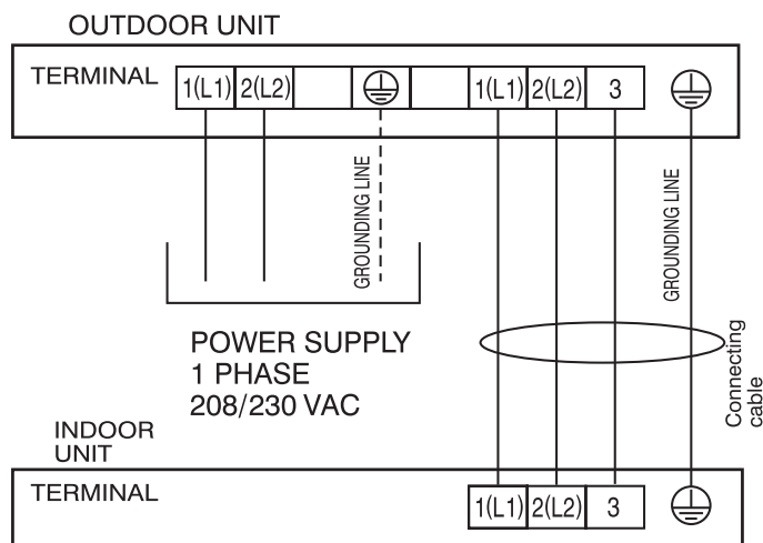
Figure 20: Terminal Block Wiring Diagram LS180HEV2, LS240HEV2.
