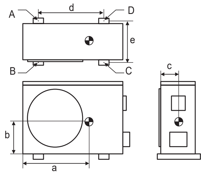
Figure 3: LSU090-120-180-240HEV2 Outdoor Unit Corner Weight and Center of Gravity Dimensions.
