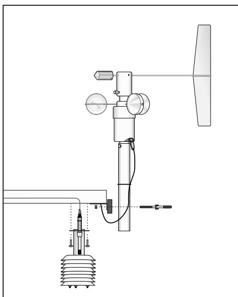
FIGURE 4.4-1. Wind and RH/Temperature Sensor Installation
