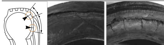
Sidewall damage due to run flat or severe under inflation
