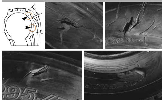
Sidewall damage due to run flat or severe under inflation
