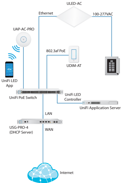
Sample Network Diagram - Wired Topology
