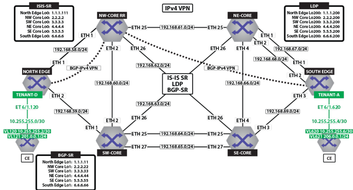
Figure 86: Tenant-D IPv4 VPN
