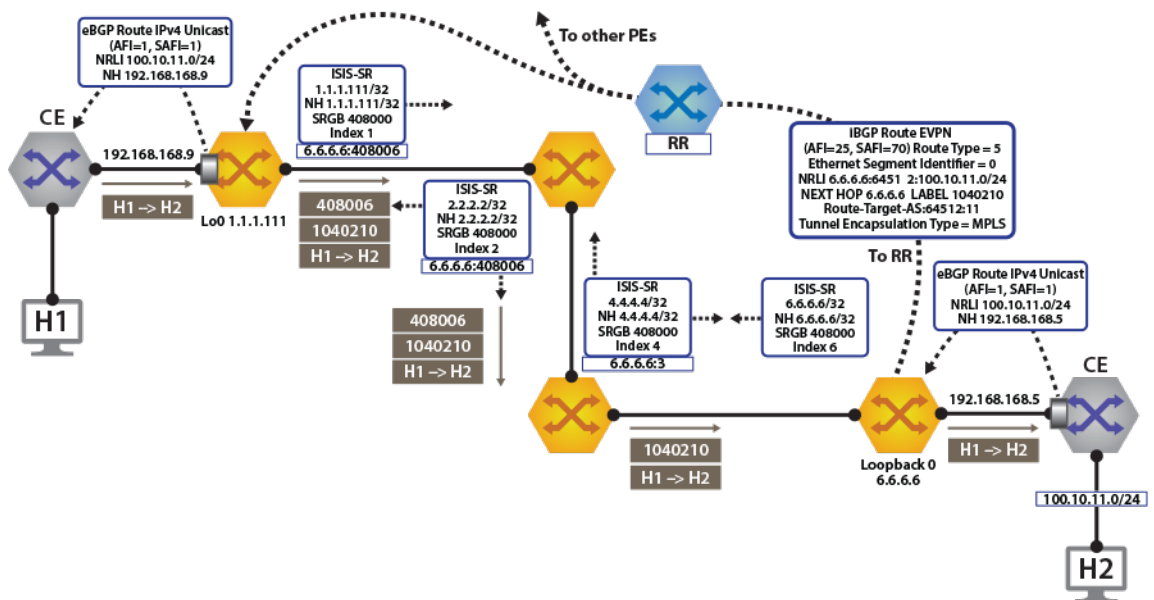
Figure 103: Control Plane & Forwarding Tenant-a Over ISIS-SR
