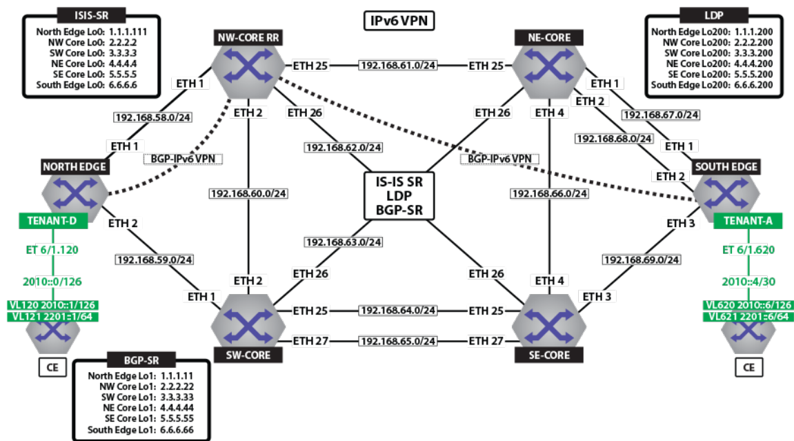
Figure 87: Tenant-D IPv6 VPN
