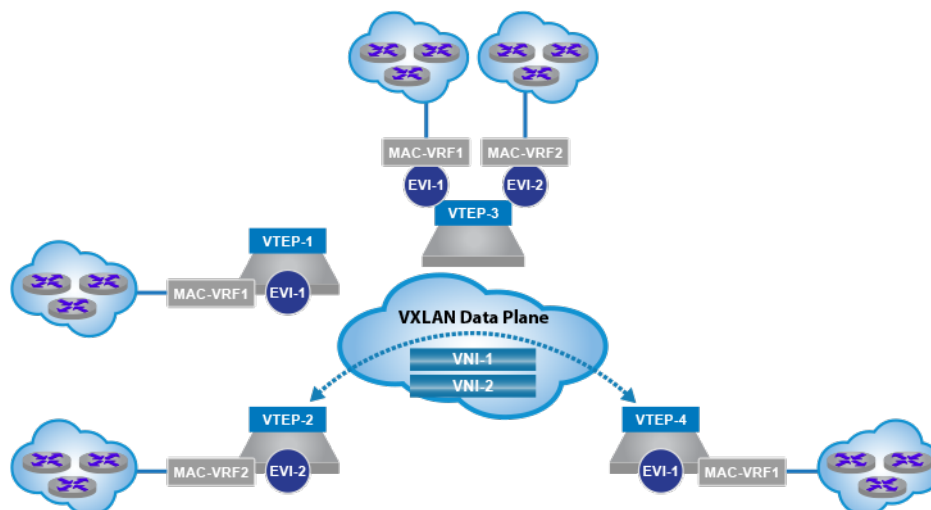
Figure 56: EVPN Terminology for a VXLAN Data Plane
