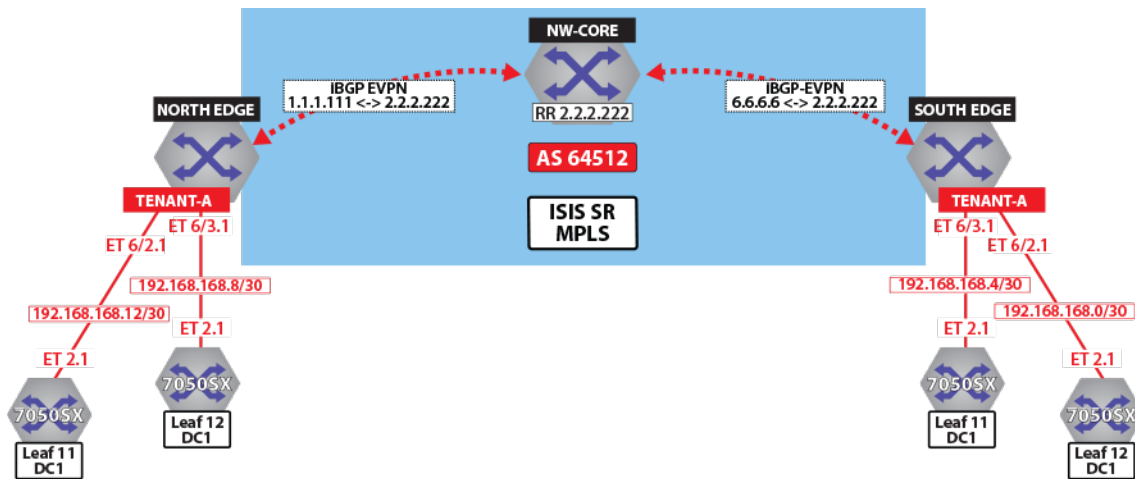
Figure 104: Control Plane Tenant-A Over LDP
