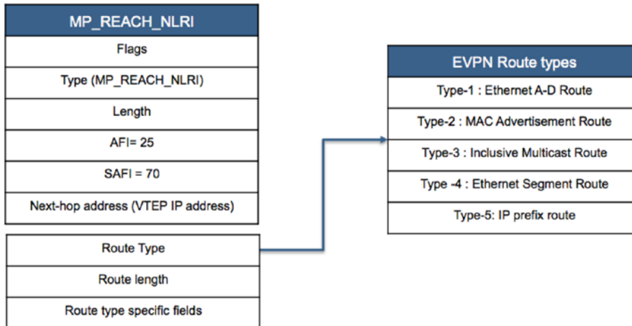
Figure 57: EVPN NLRI Route Format
