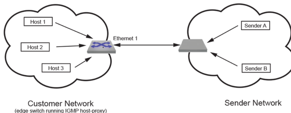
Figure 47: IP IGMP Host Proxy Implementation
