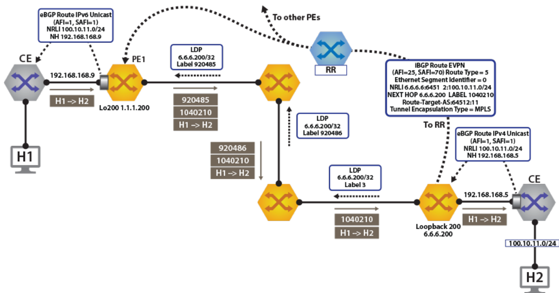
Figure 106: Control Plane & Forwarding Tenant-a Over LDP
