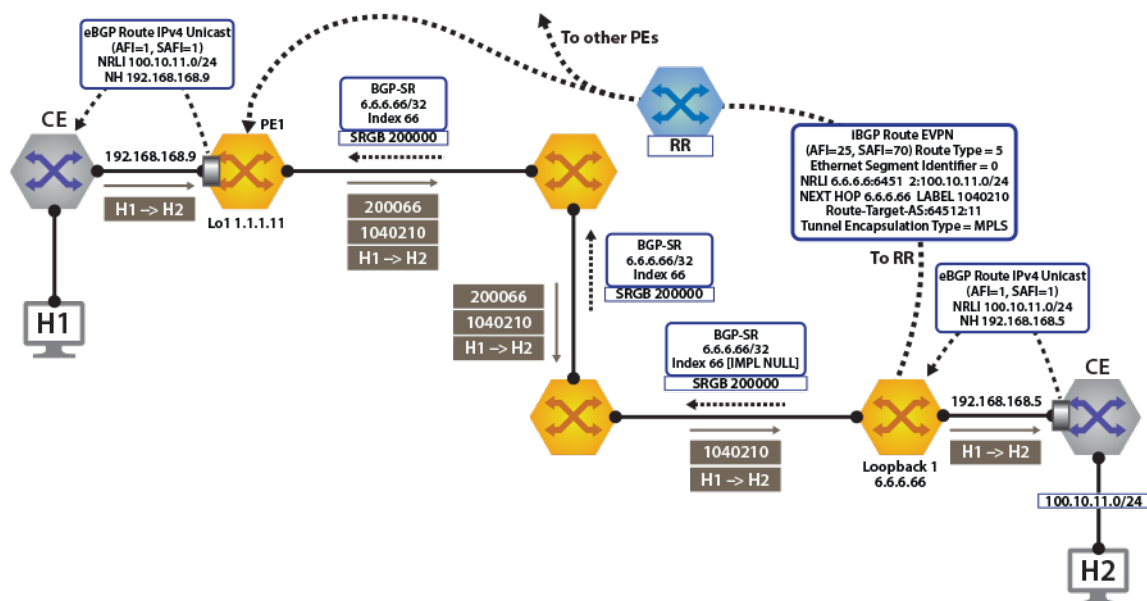
Figure 109: Control Plane & Forwarding Tenant-a Over BGP-SR
