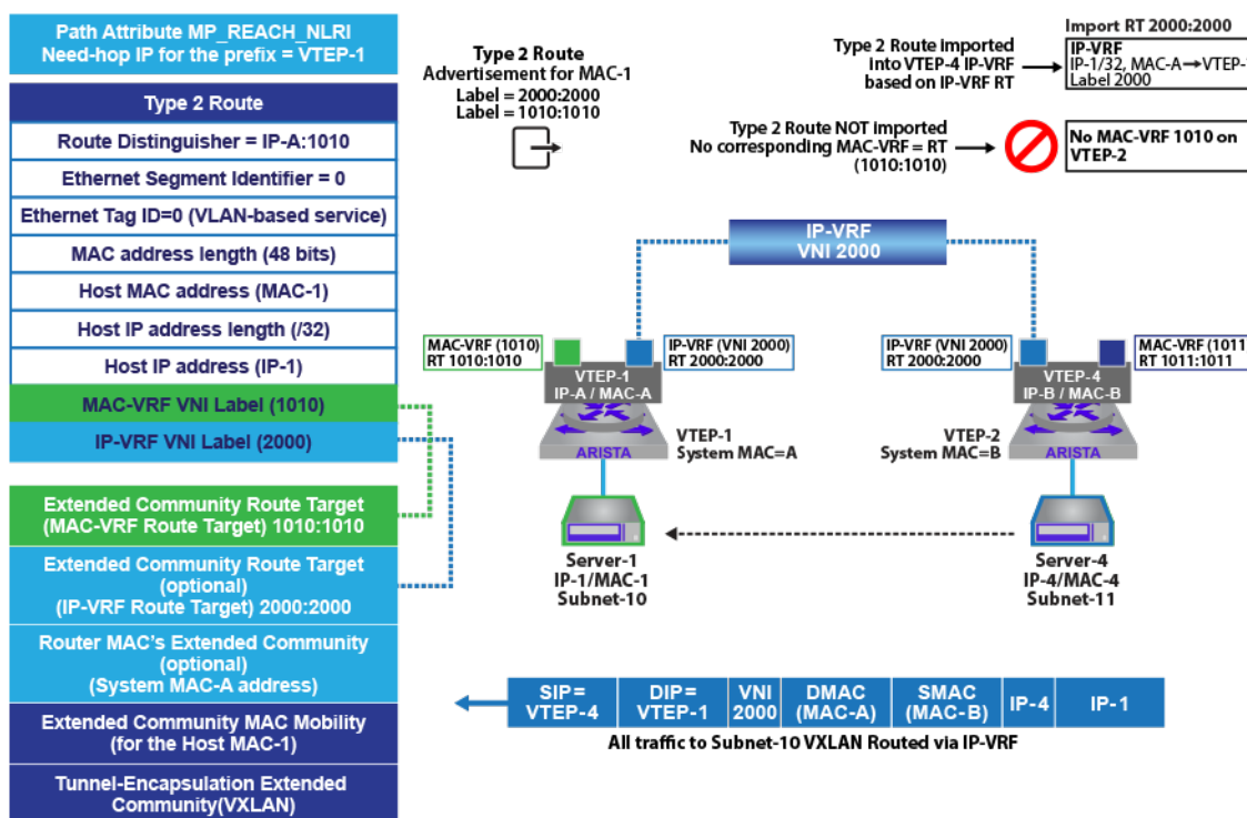
Figure 75: EVPN Type 2 Route in Symmetric IRB - MAC-VRF Only Exists on Sending VTEP
