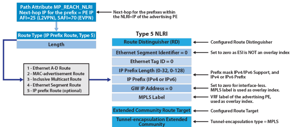
Figure 92: EVPN Route Type-5, for Advertisement of IP Prefixes
