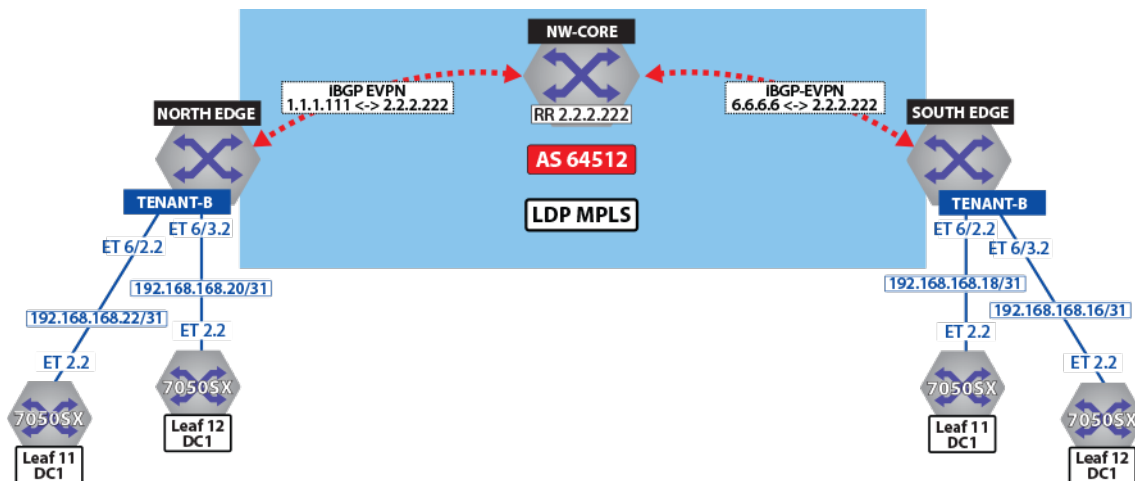
Figure 105: Control Plane Tenant-B over LDP
