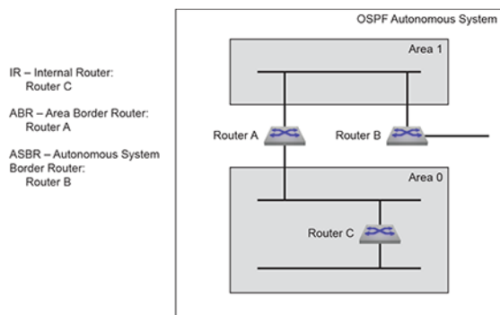
Figure 31: OSPFv2 Router Types
