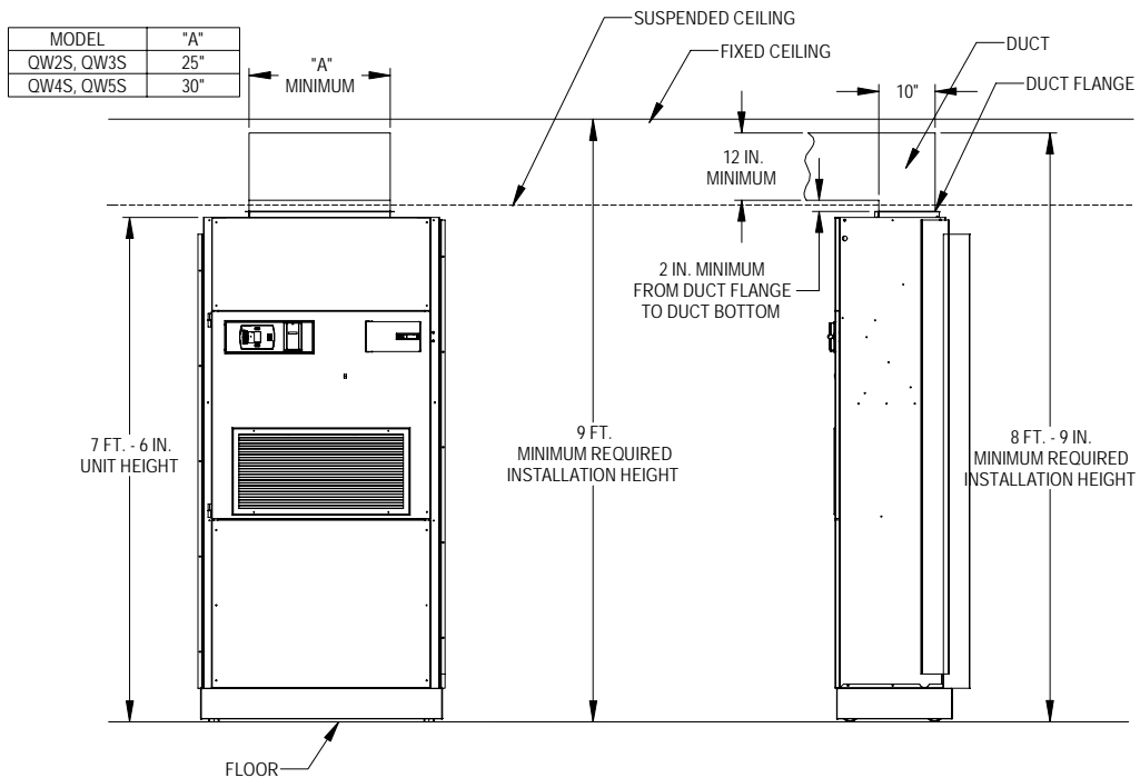
FIGURE 6 Ducted Application
