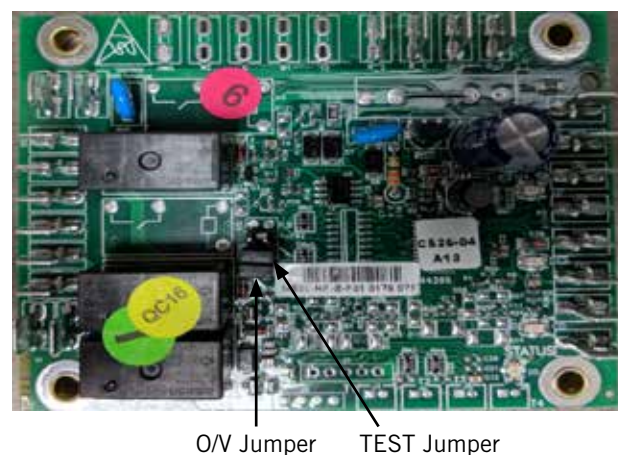
FIGURE 22 Geothermal Compressor Logic Control Board
