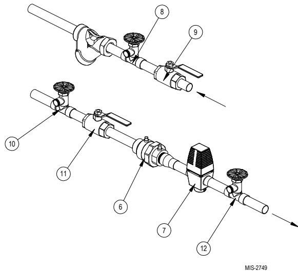
Figure 33 Piping Diagram
