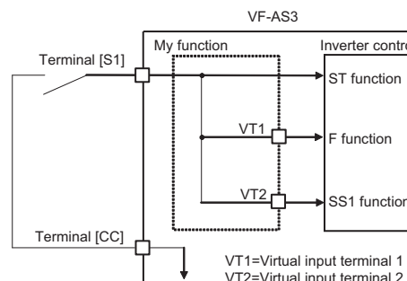
Fig. 5-6 Block diagram for Example 3
