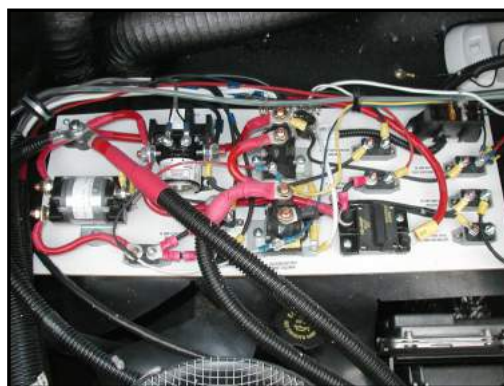
Figure 7-10. Circuit Breakers
