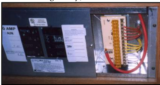
Figure 7-1. Circuit-Breaker Box
