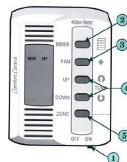
Figure 3-2. Thermostat Details
