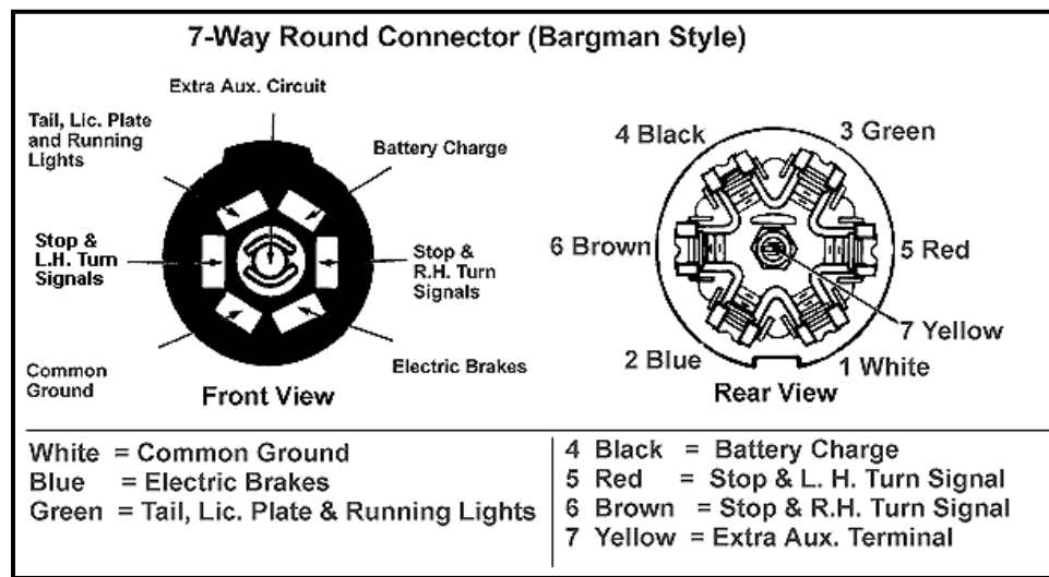
Figure 7-13. Seven-Pin Towing Connector
