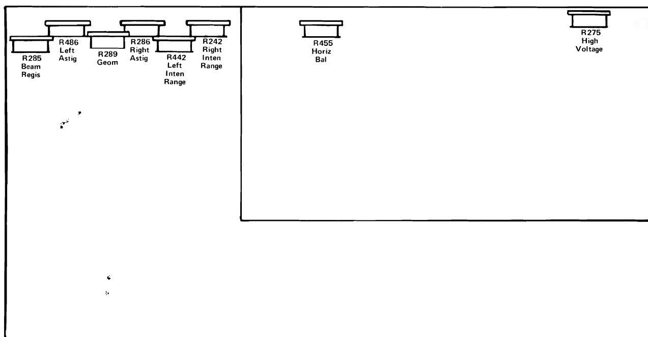
Fig. 4-4. Location of CRT Circuit adjustments.
