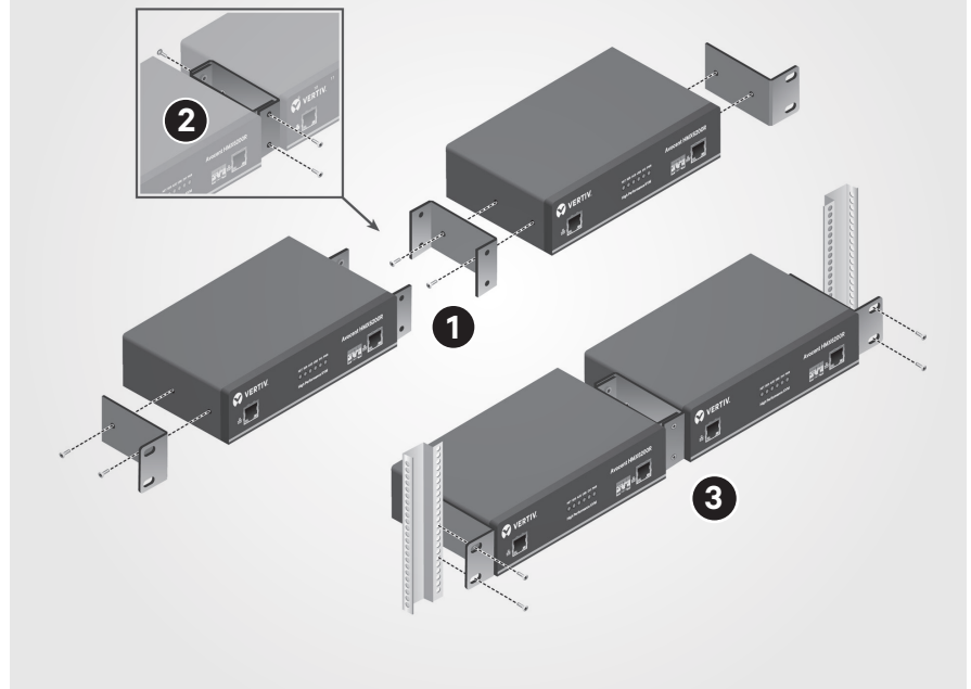
Dual Unit Mounting (HMX extender shown)
