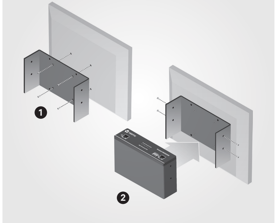
Single Unit Mounting (HMX extender shown)
