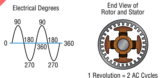
Figure 9 – A Four-Pole Alternator-Type Design
