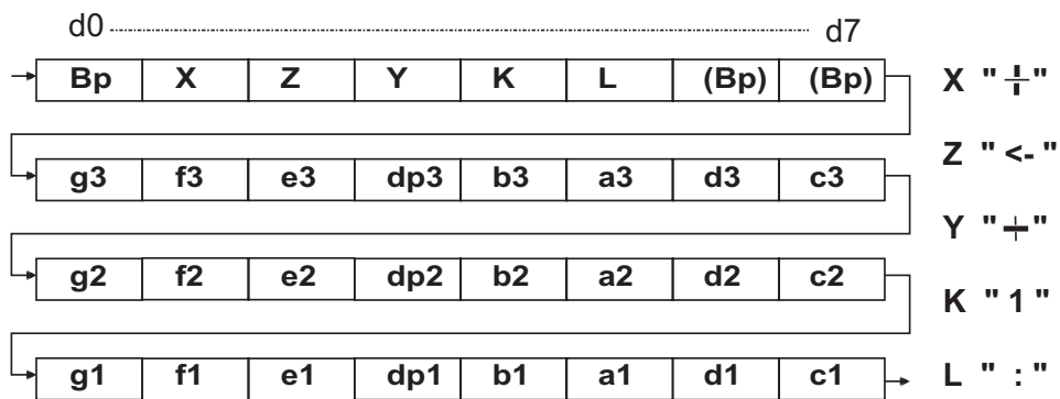
7 segment codes for all digits
