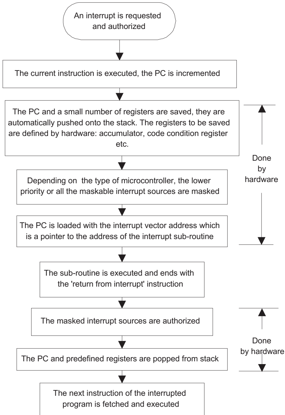
Interrupt processing flowchart
