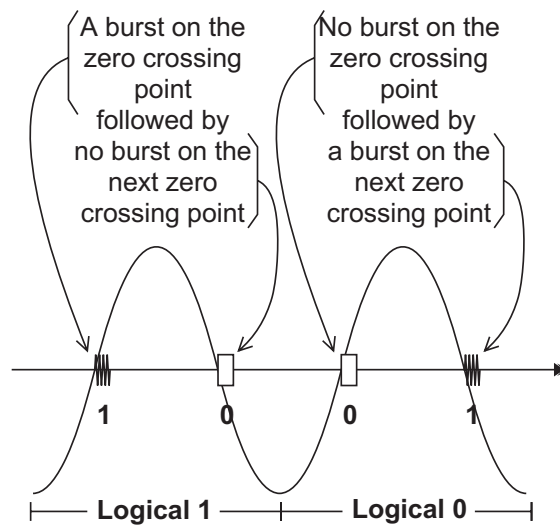
X-10 Technology : bit transmission principle (House & Key codes, except Start code)
