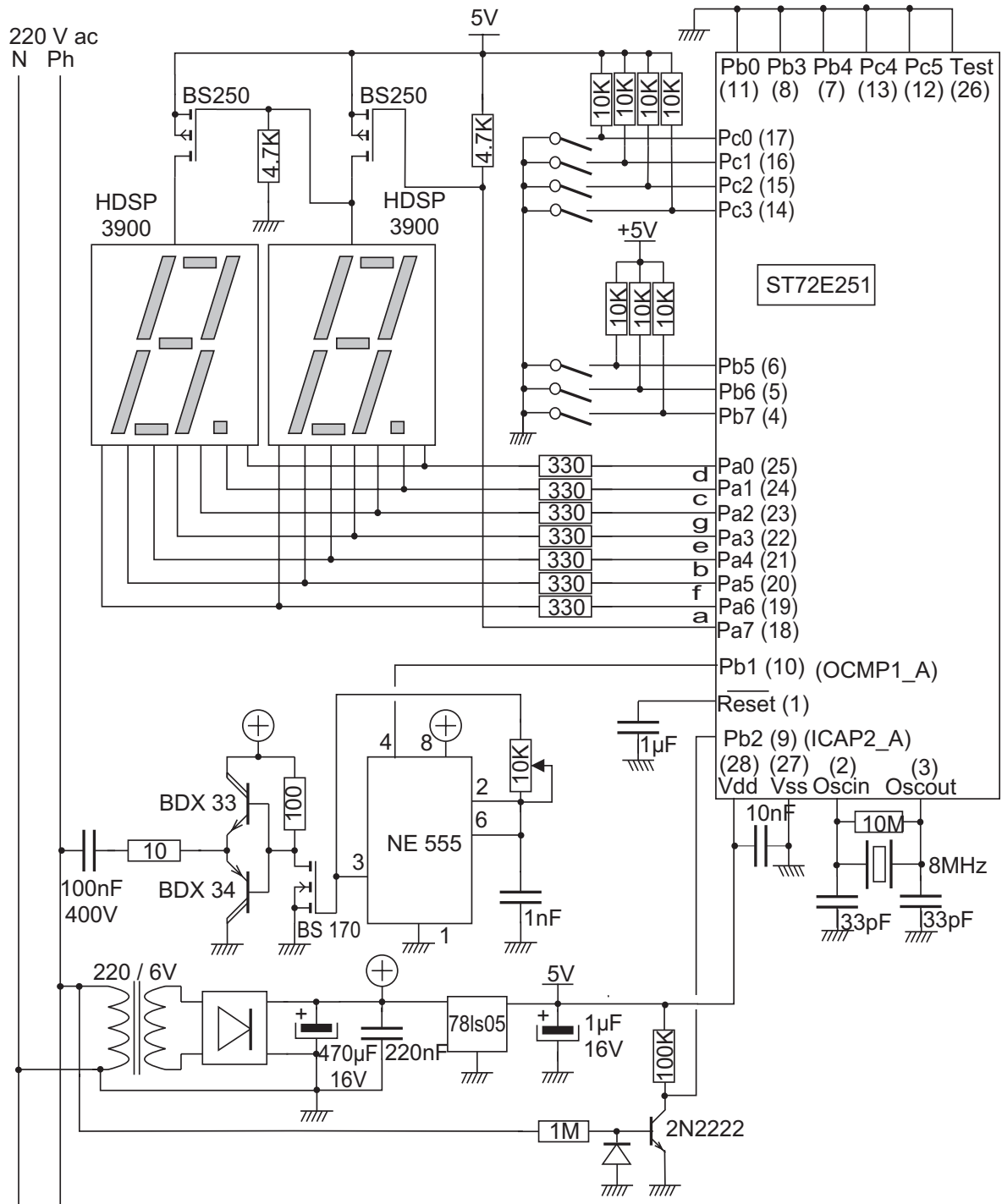
Carrier-current system : diagram of the transmitter circuit
