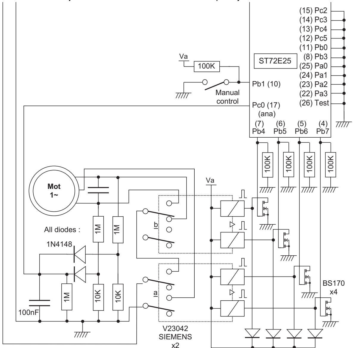
Carrier-current system : diagram of the receiver circuit ;
