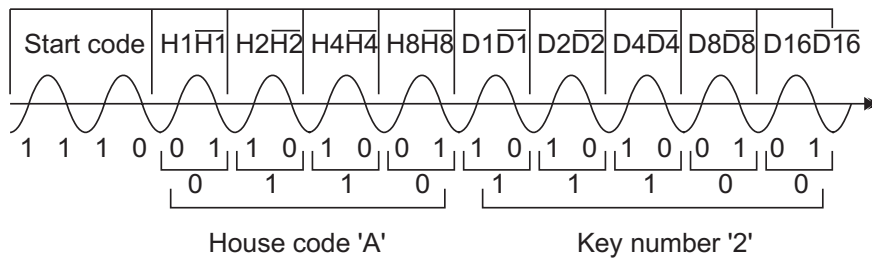
X-10 Technology :Transmission example
