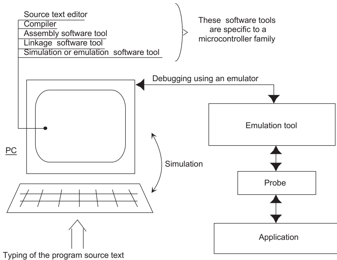
PC-based development environment
