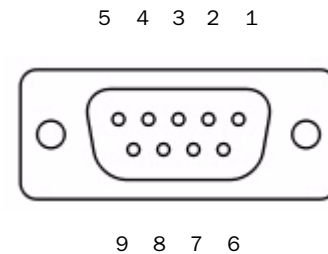
Pinout for VENUE SC48 DB9 GPI port (looking at back of console)
