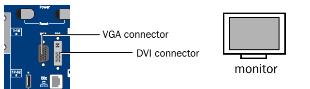
VGA and DVI display connectors on the back panel
