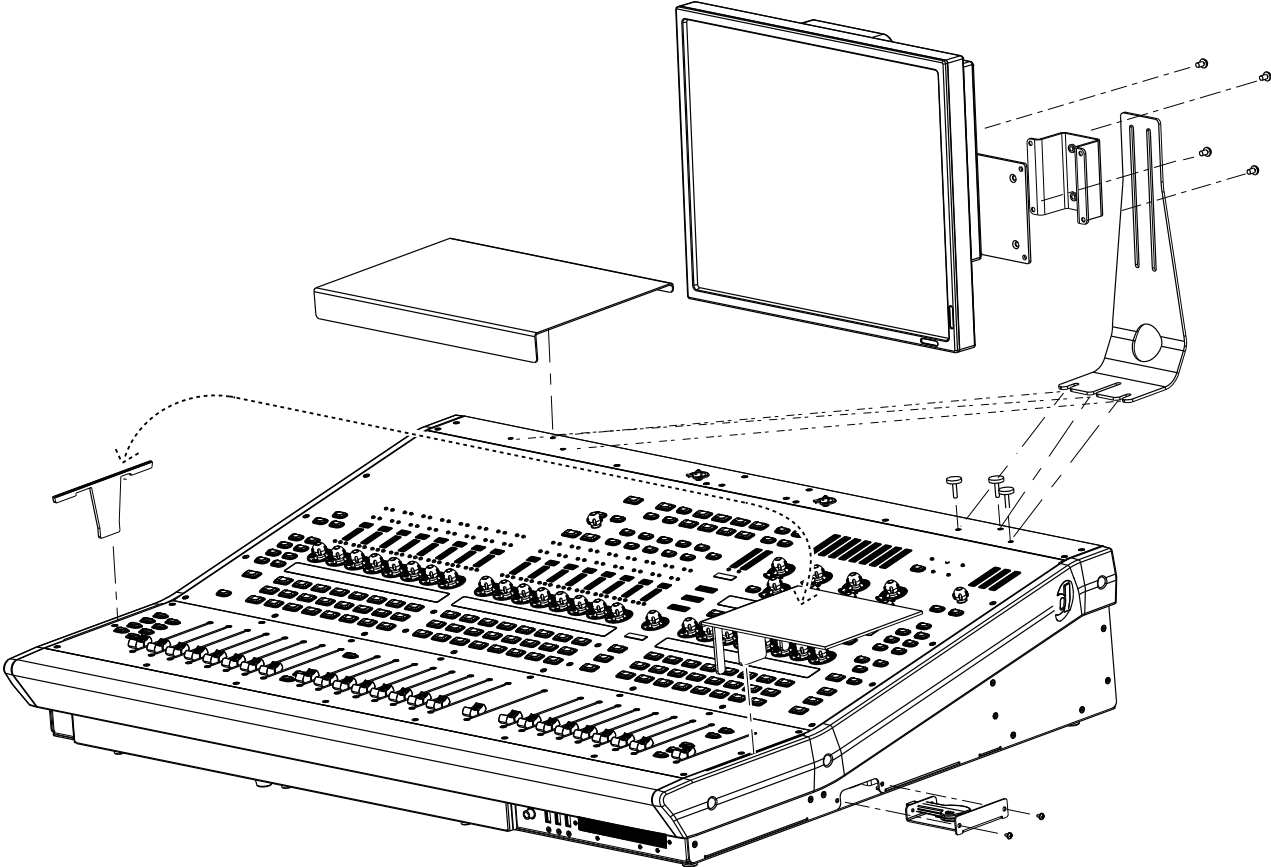
Figure 2. Video Mount, Mouse Tray and Accessory Tray
