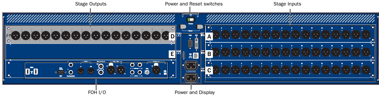
Figure 3. Back panel
