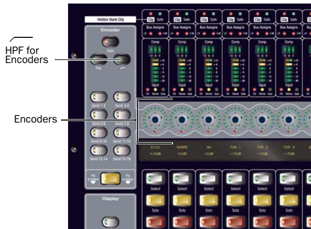
HPF controls for Input Channels
