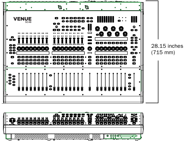
Dimensions, VENUE SC48
