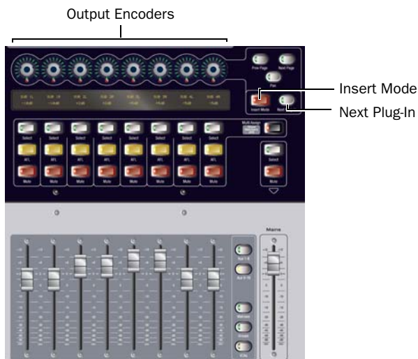
Encoders, Insert mode and Next Plug-In switches in the Output section
