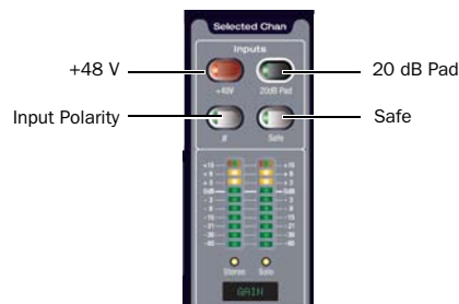
Input controls in the ACS
