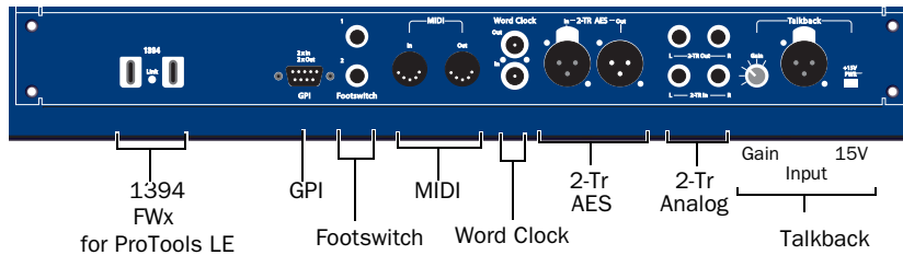
Figure 6. FOH connectors and controls
