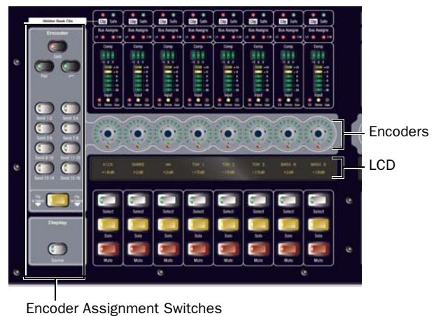
Encoder Assignment Switches
