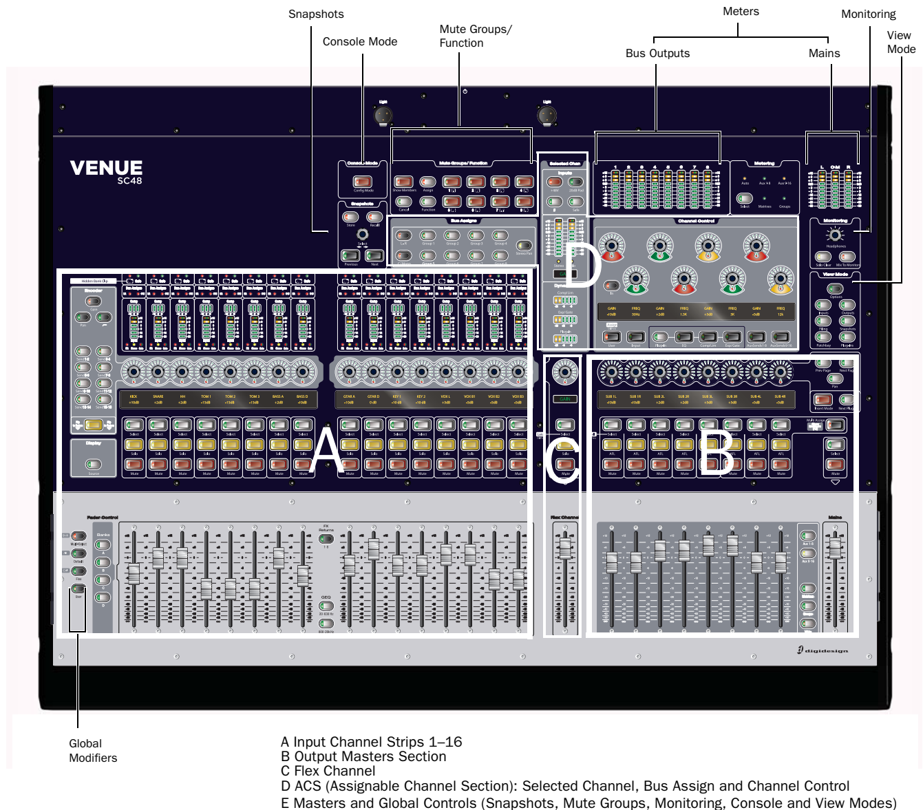
Figure 7. Main control sections on VENUE SC48
