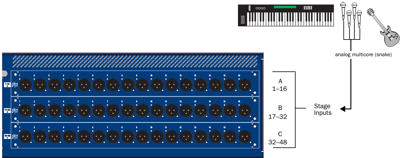
Figure 4. SC48 I/O slots A–C for stage inputs 1–48
