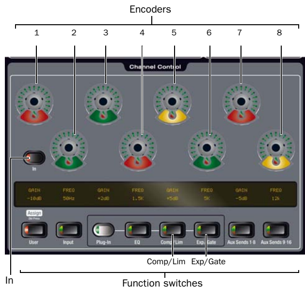
Controls for built-in dynamics processors in Channel Control
