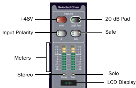
Selected Channel Input controls, meters and displays
