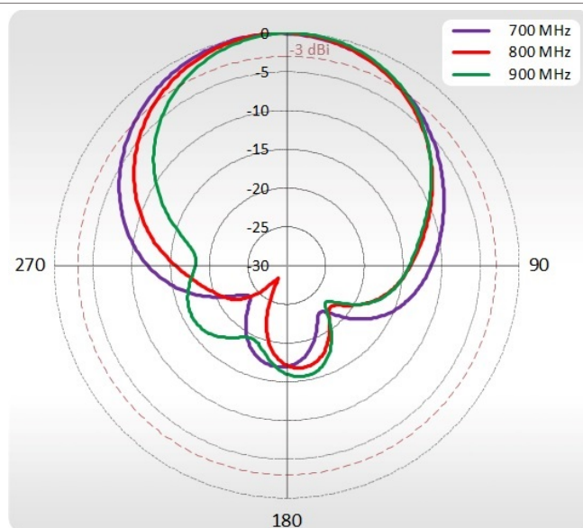
Port 2 700-900 MHz Elevation
