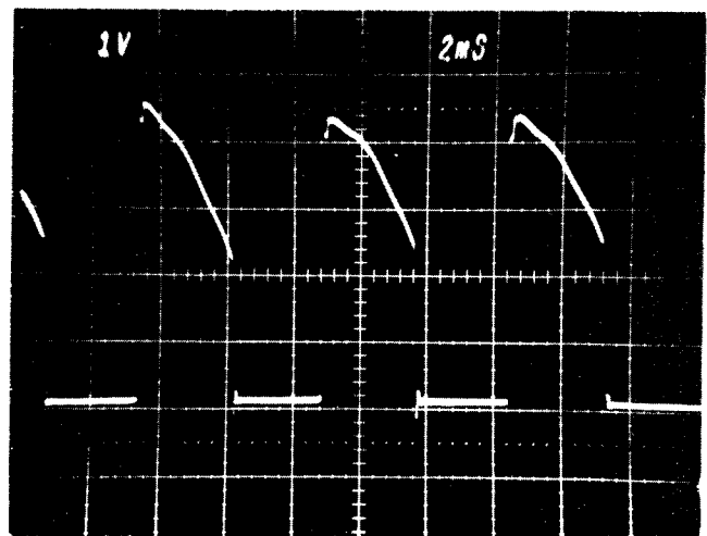
Figure A. Prototype GENERREX* excitation system generator field voltage
