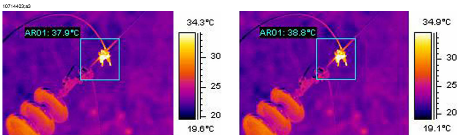
Figure 13.18 LEFT: Incorrect distance setting; RIGHT: Correct distance setting
