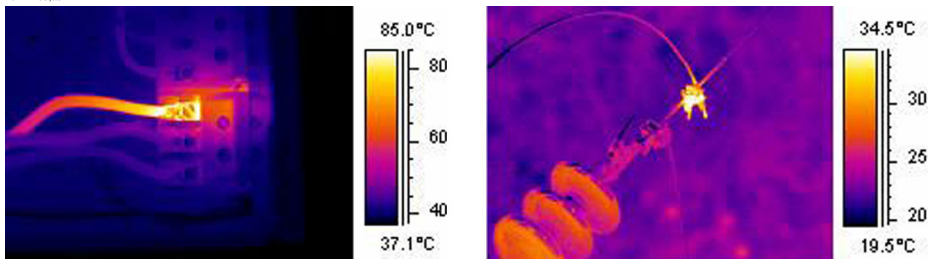
Figure 13.16 LEFT: An infrared image showing bad contact due to a loose bolt; RIGHT: A loose outdoor connection, exposed to the wind cooling effect.
